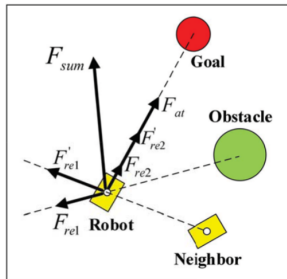
(a) Attractive and repulsive forces acting on an agent in a multi-robot setting [30].
