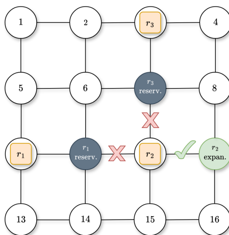
Figure 5.9: TEA* expansion step illustrating two reservation-based rejections.
