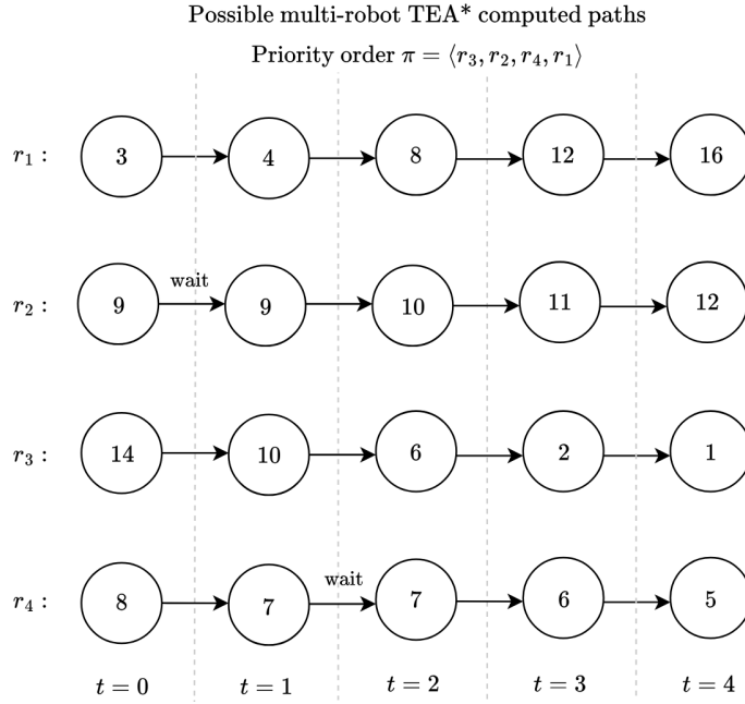
Figure 5.8: Possible TEA* plan obtained with the weighted conflict ordering.
