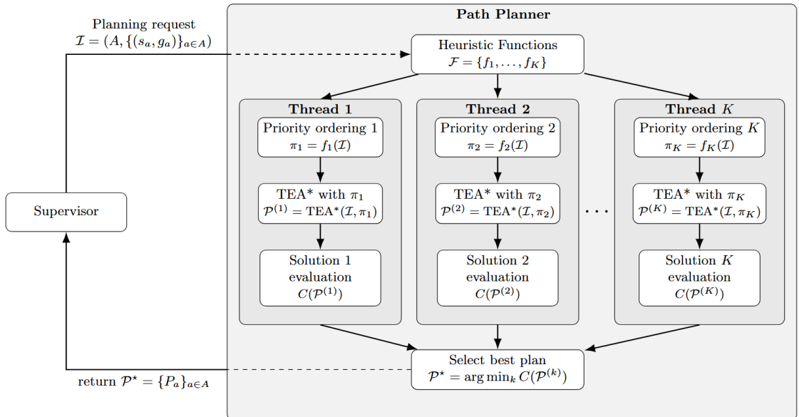
Figure 4.1: Conceptual overview of the proposed preliminary multithreaded planning approach.
