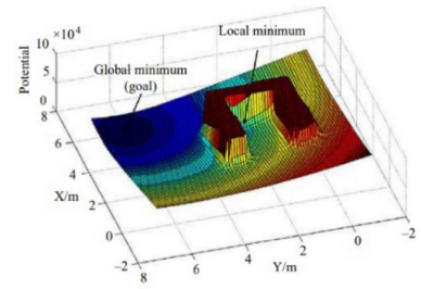
(c) Potential field exhibiting local minima induced by obstacles [31].
