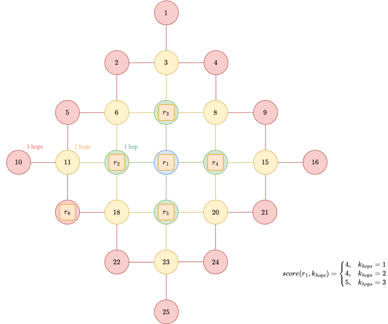
Figure 5.5: Illustration of the K-hop Neighbour Density heuristic. The score of robot r_1 depends on the number of robots located within the graph neighbourhood defined by k_{\text{hops}} .
