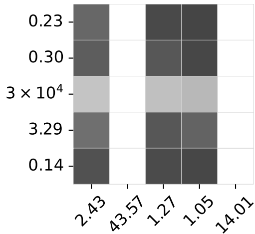
\tilde{W}^{(2)}
