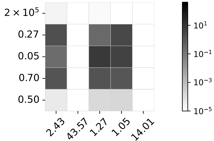
\tilde{W}^{(3)}
