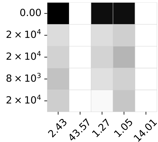
\tilde{W}^{(1)}
