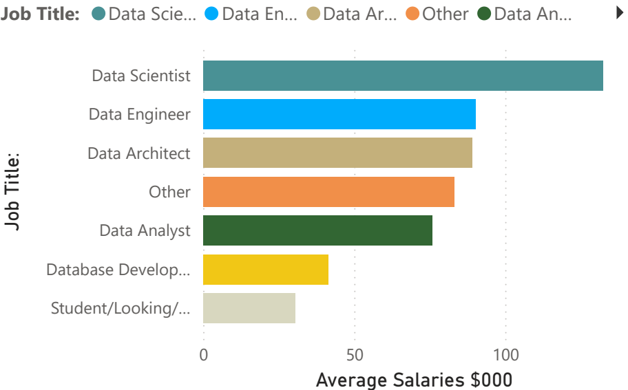
Average Salaries ($000) of Various Data Professionals
