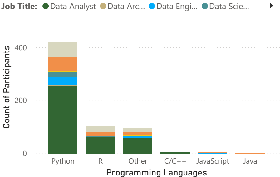
Popular Programming Languages in Various Professions
