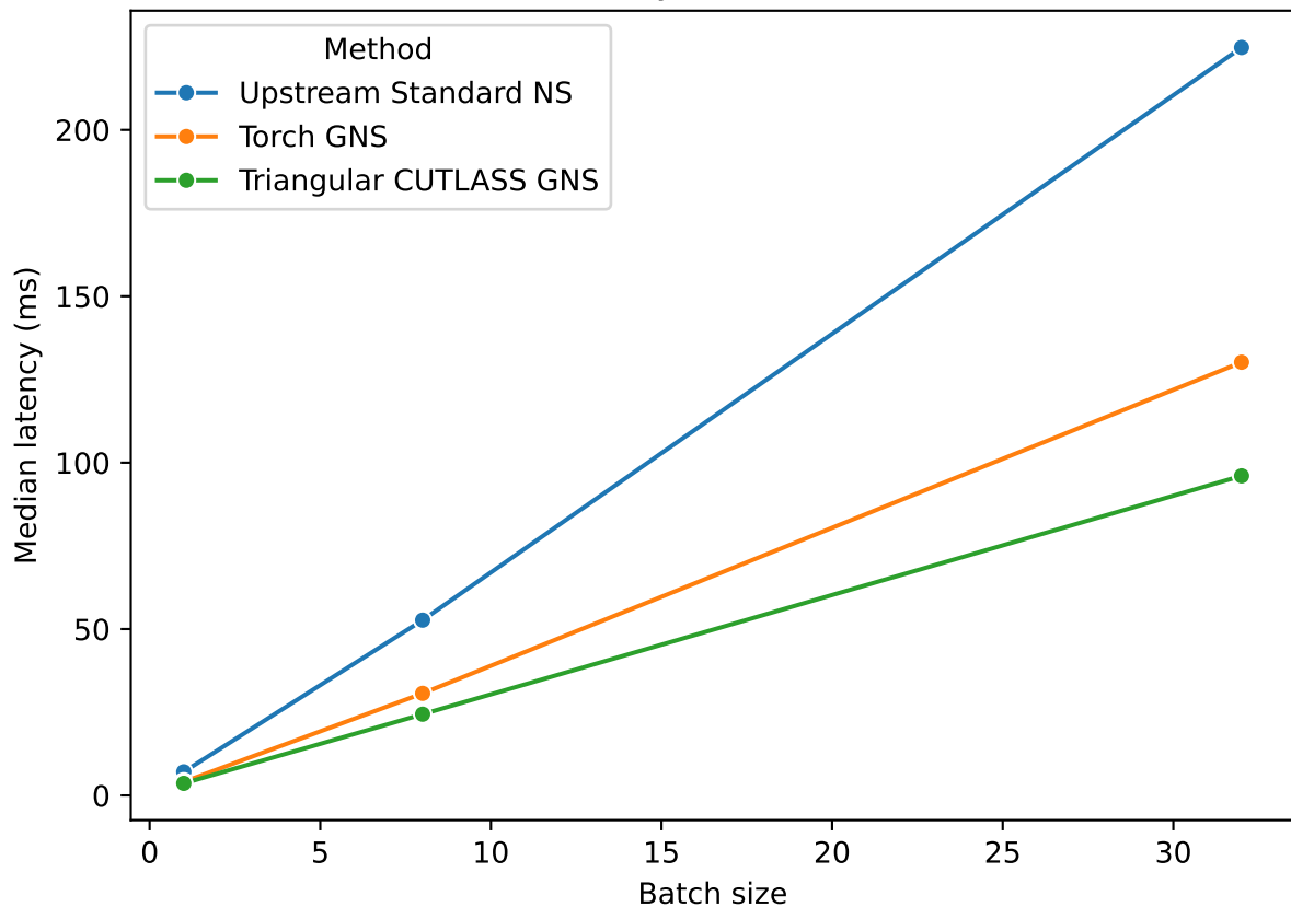
One-A100 latency at B \times 16384 \times 2048
