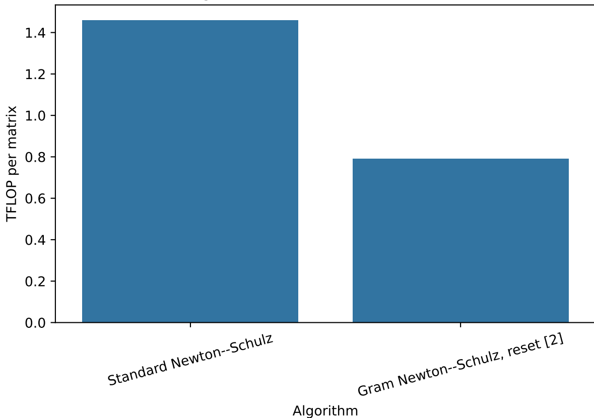
Algorithmic work at 16384 \times 2048
