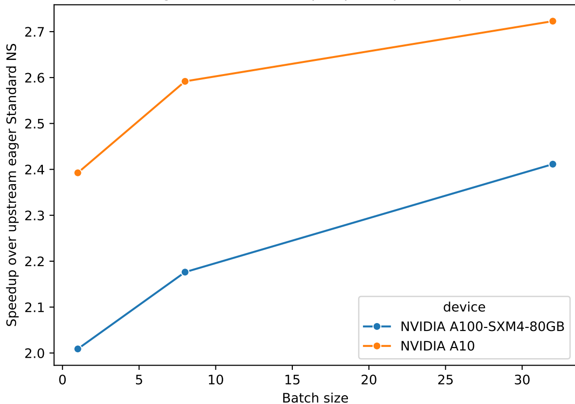
Single-GPU actual-shape speedup on Ampere
