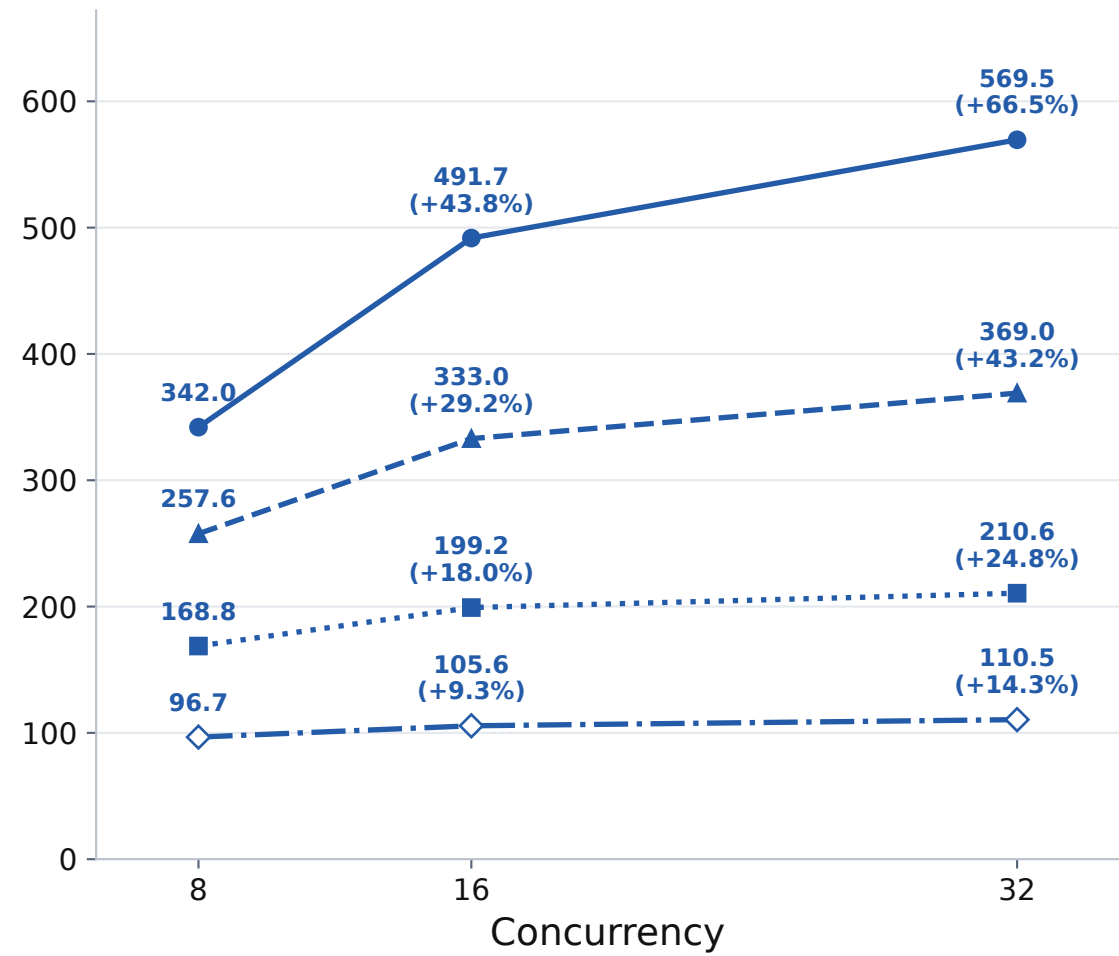
Q4_K_M
