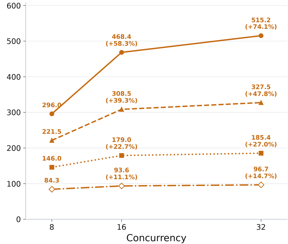
Q2_K
