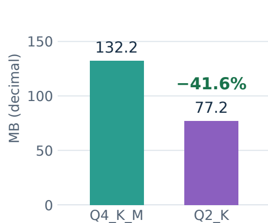
DRAM reads
