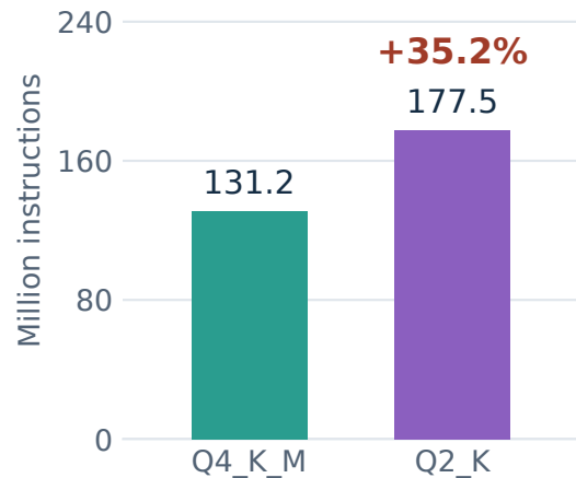
Executed instructions
