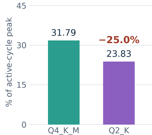
Achieved occupancy
