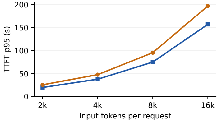
(b) First-token latency
