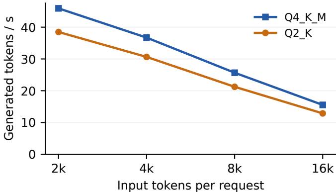
(a) Aggregate output throughput
