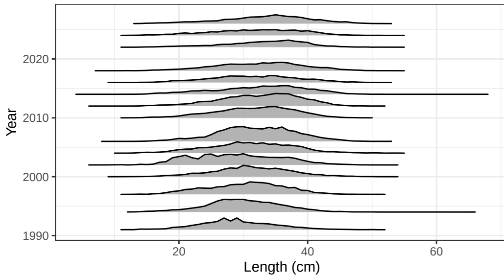
Figure 8.3.: AI Rock sole size compositions and ridge plot.
