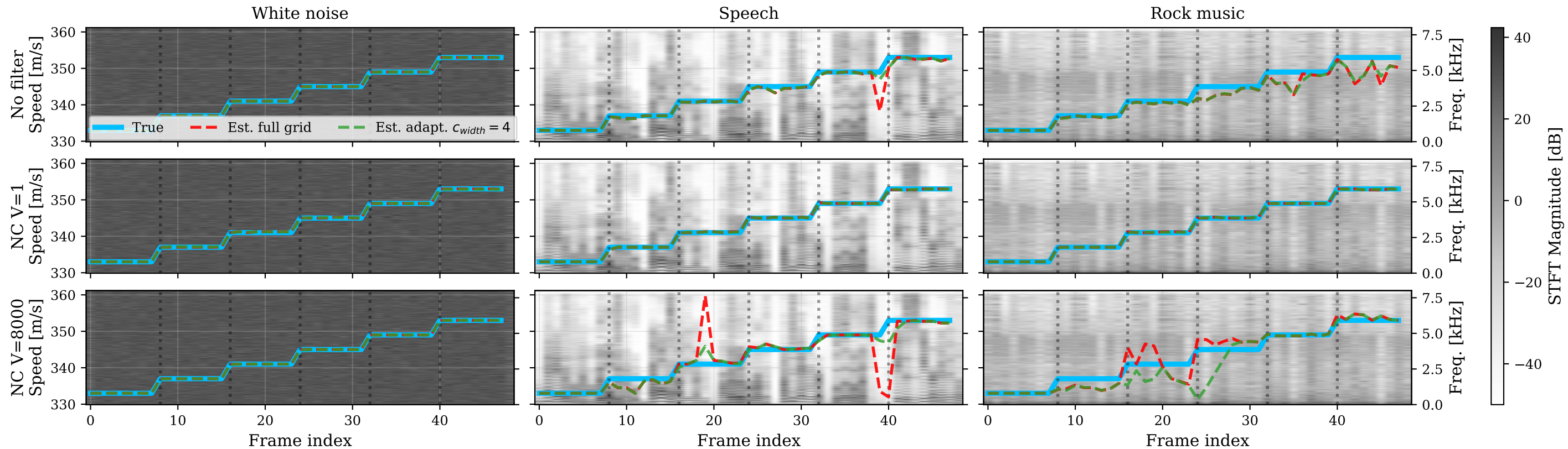
Speed tracking - From 333m/s to 353 m/s - Speed Change: 4m/s, \Delta t=2s (16 active LSPs)
