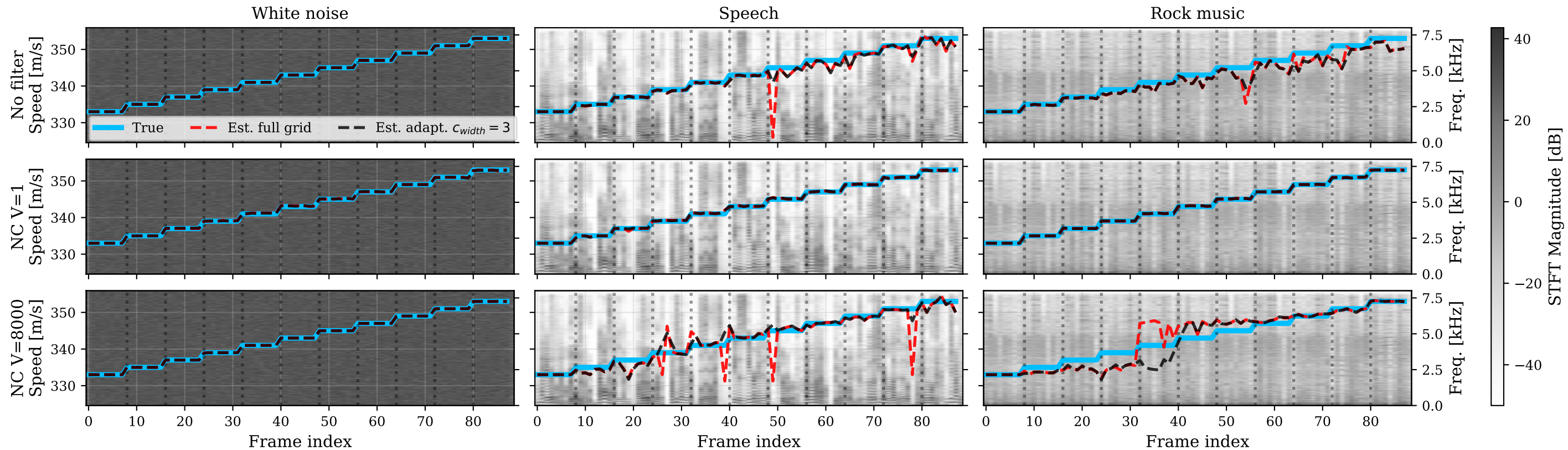
Speed tracking - From 333m/s to 353 m/s - Speed Change: 2m/s, \Delta t=2s (16 active LSPs)
