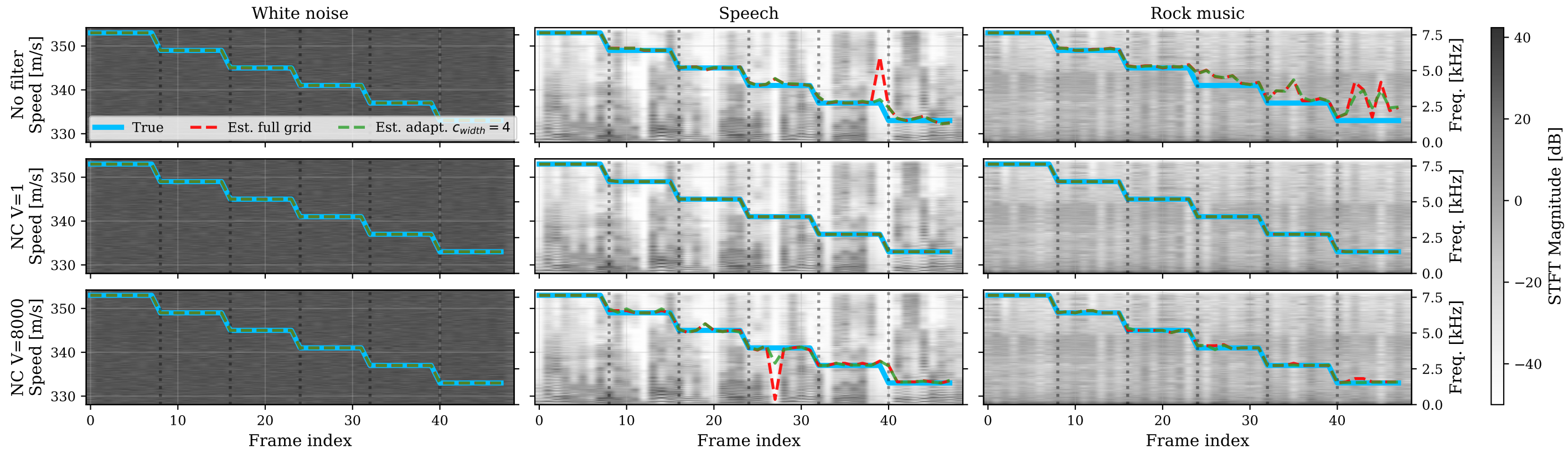
Speed tracking - From 353m/s to 333 m/s - Speed Change: 4m/s, \Delta t=2s (16 active LSPs)
