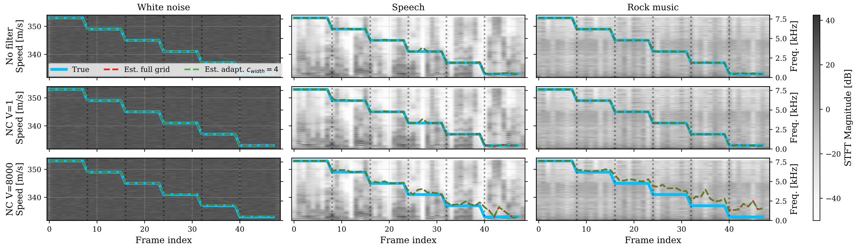
Speed tracking - From 353m/s to 333 m/s - Speed Change: 4m/s, \Delta t=2s (1 active LSP)
