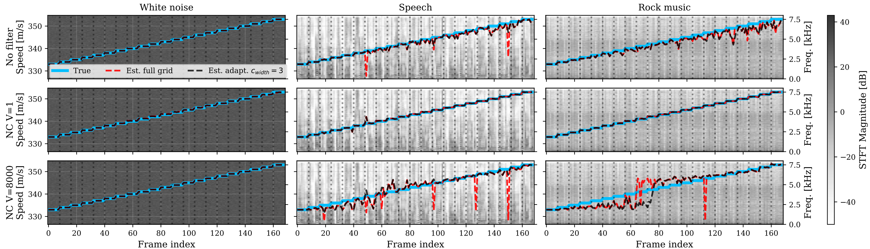
Speed tracking - From 333m/s to 353 m/s - Speed Change: 1m/s, \Delta t=2s (16 active LSPs)
