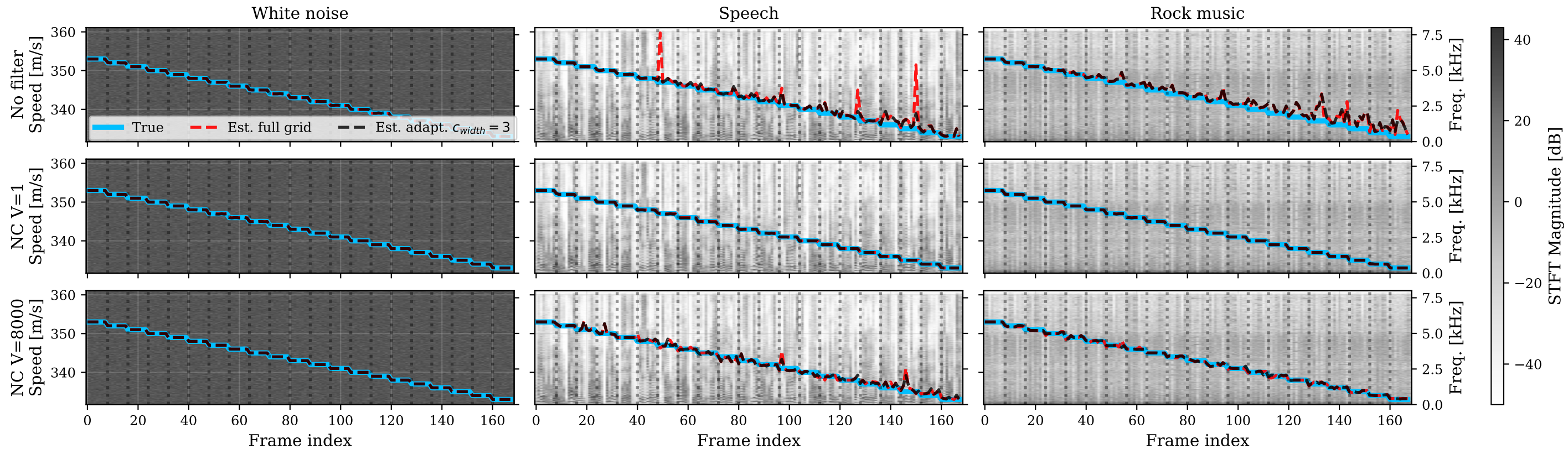
Speed tracking - From 353m/s to 333 m/s - Speed Change: 1m/s, \Delta t=2s (16 active LSPs)
