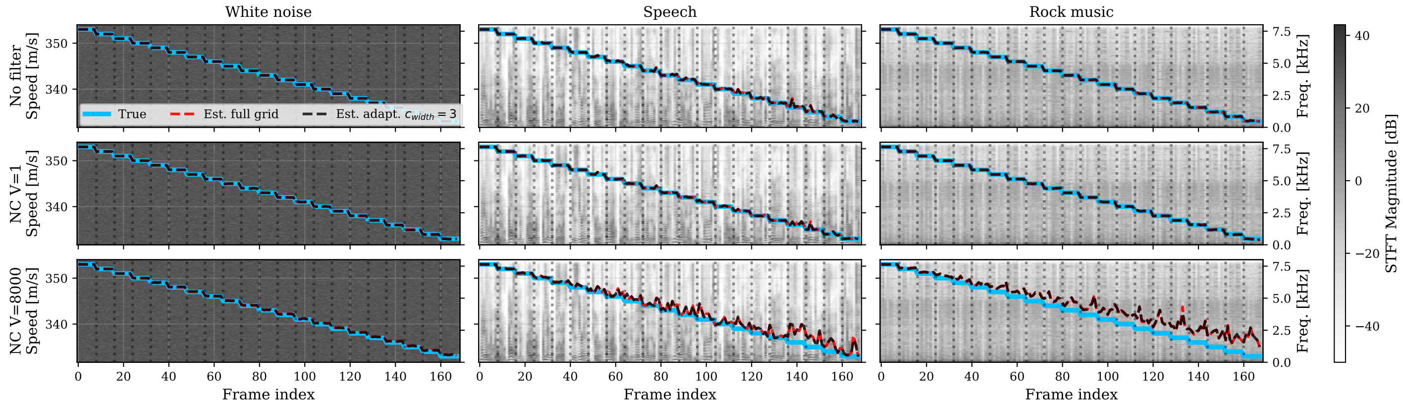
Speed tracking - From 353m/s to 333 m/s - Speed Change: 1m/s, \Delta t=2s (1 active LSP)
