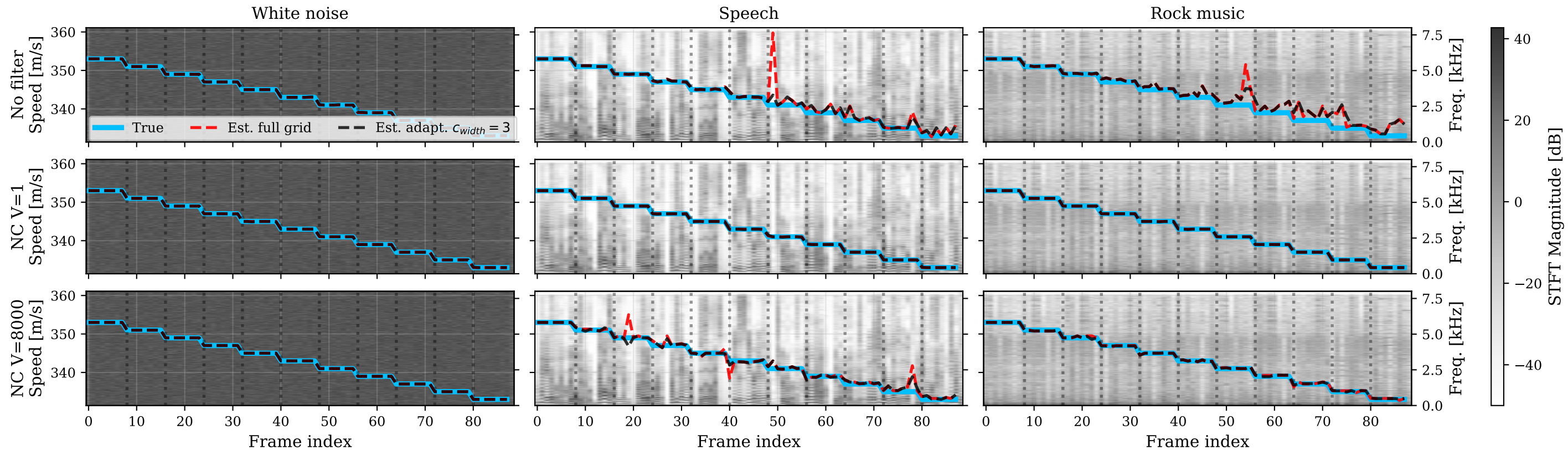
Speed tracking - From 353m/s to 333 m/s - Speed Change: 2m/s, \Delta t=2 s (1 active LSP)
