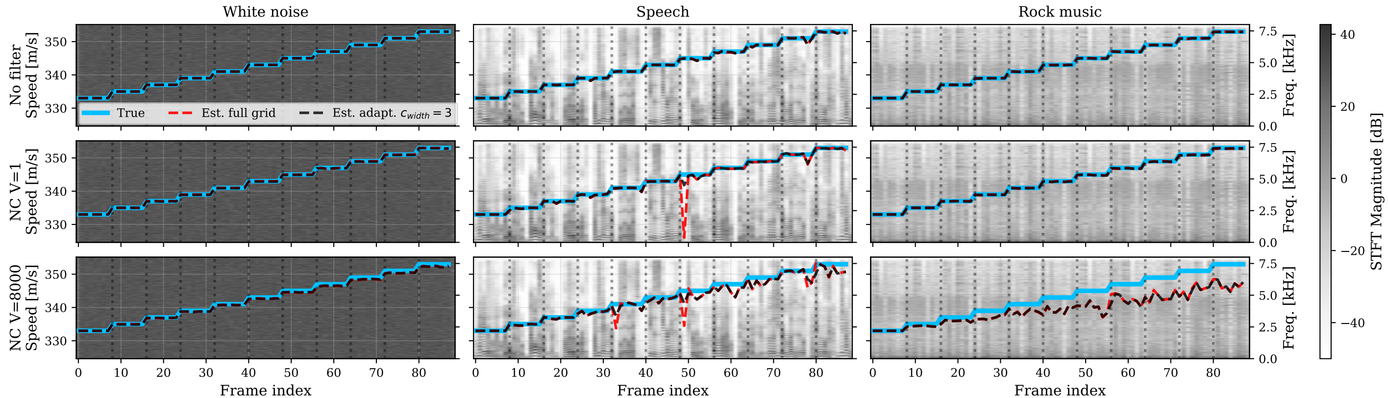
Speed tracking - From 333m/s to 353 m/s - Speed Change: 2m/s, \Delta t=2 s (1 active LSP)
