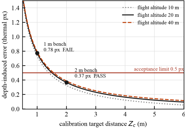
Fig. 4. Depth-induced reprojection error from (9) for the measured 27 mm baseline. The acceptance limit is 0.5 thermal px. A 1 m bench calibration cannot meet it at any operating altitude; 2 m can. The curve flattens beyond about 3 m, so there is no benefit in a longer and more awkward standoff.
