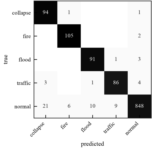
Fig. 6. Scene classifier confusion matrix, 1,286 validation images, shaded by row-normalised rate and annotated with counts. Off-diagonal mass lies almost entirely in the bottom row: the model over-calls hazards on normal scenes rather than missing hazards.
