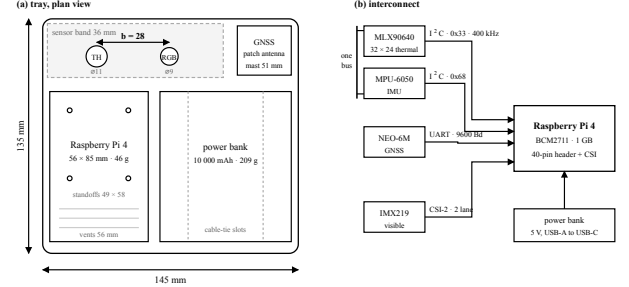
Fig. 2. Physical integration. (a) The 145 \times 135 mm printed tray in plan, sensors forward. Both sensors are located by pockets cut to their PCB outlines rather than by their mounting holes, at an optical baseline b = 28 mm; the vent slots under the Pi are 56 mm, a length derived from the microSD notch position rather than chosen. The GNSS patch antenna stands off the plate on a 51 mm mast, away from the SoC. (b) The interconnect. The thermal array and the IMU share one 400 kHz I 2 C bus at distinct addresses, the GNSS receiver has the hardware UART to itself, and the visible camera is on CSI-2, so no two sensors contend for a bus.
