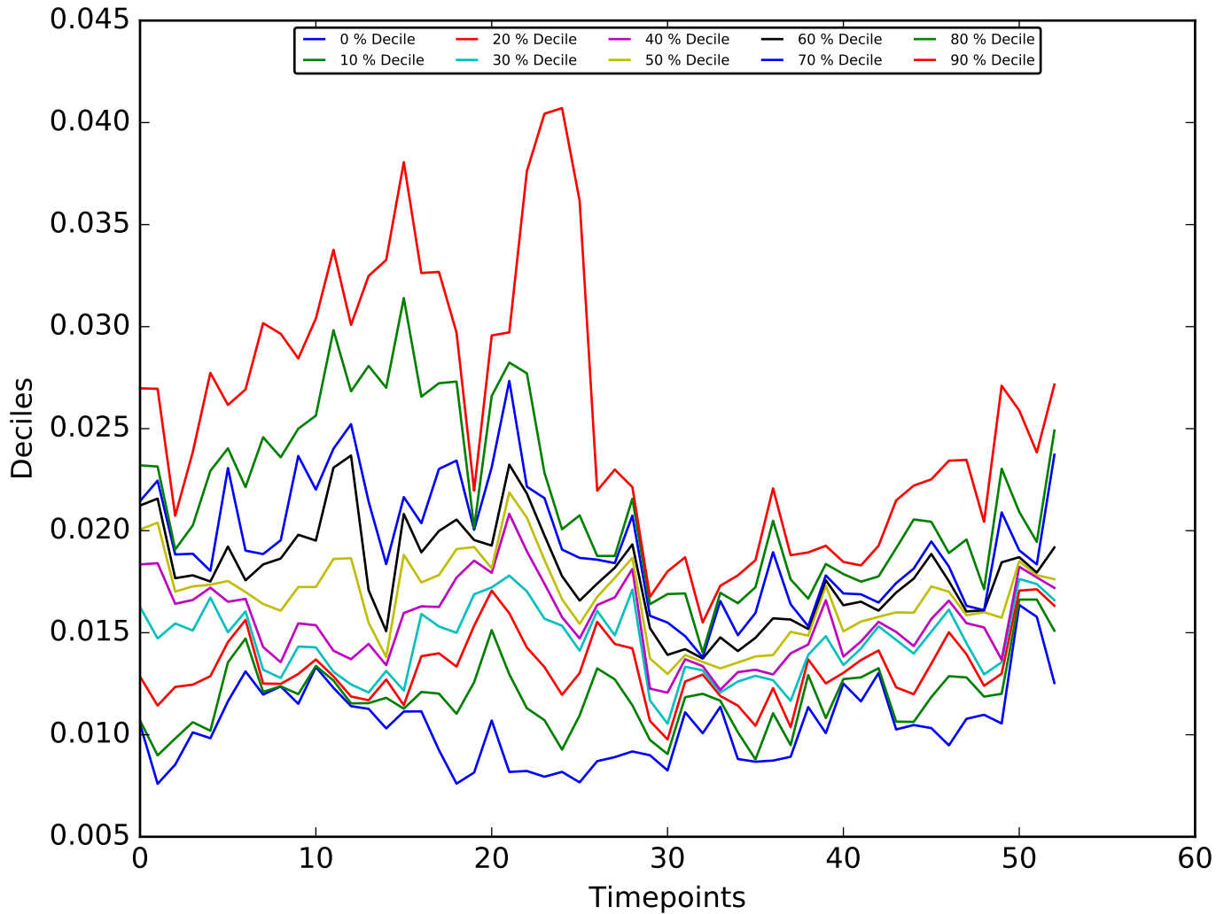
Distribution of Transition Matrix Error Along Trajectory (Naive)
