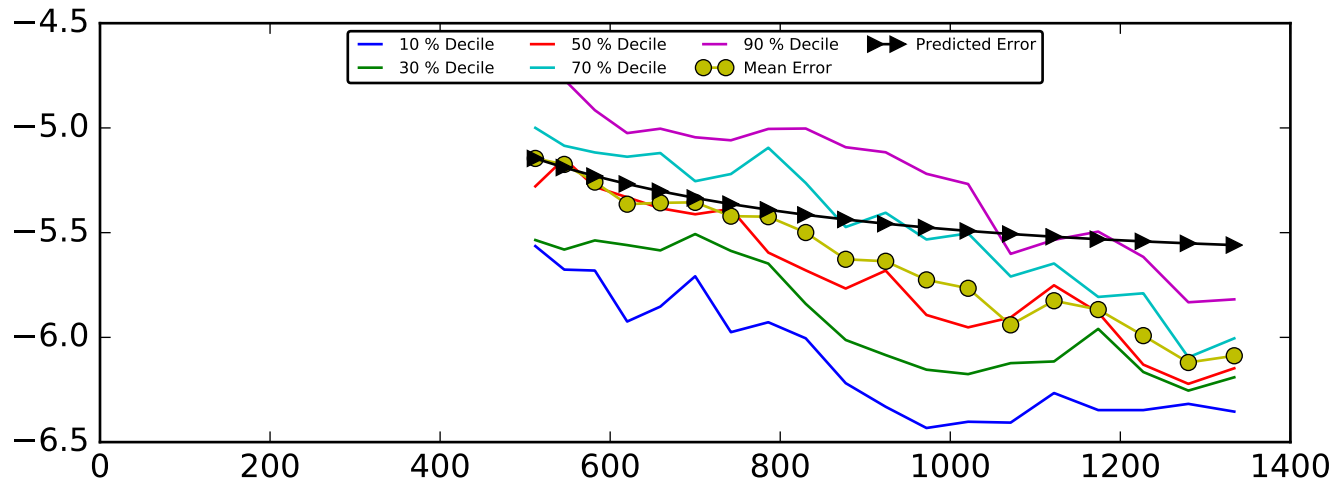
Distribution of Transition Matrix Error Along Trajectory (Bayes)
