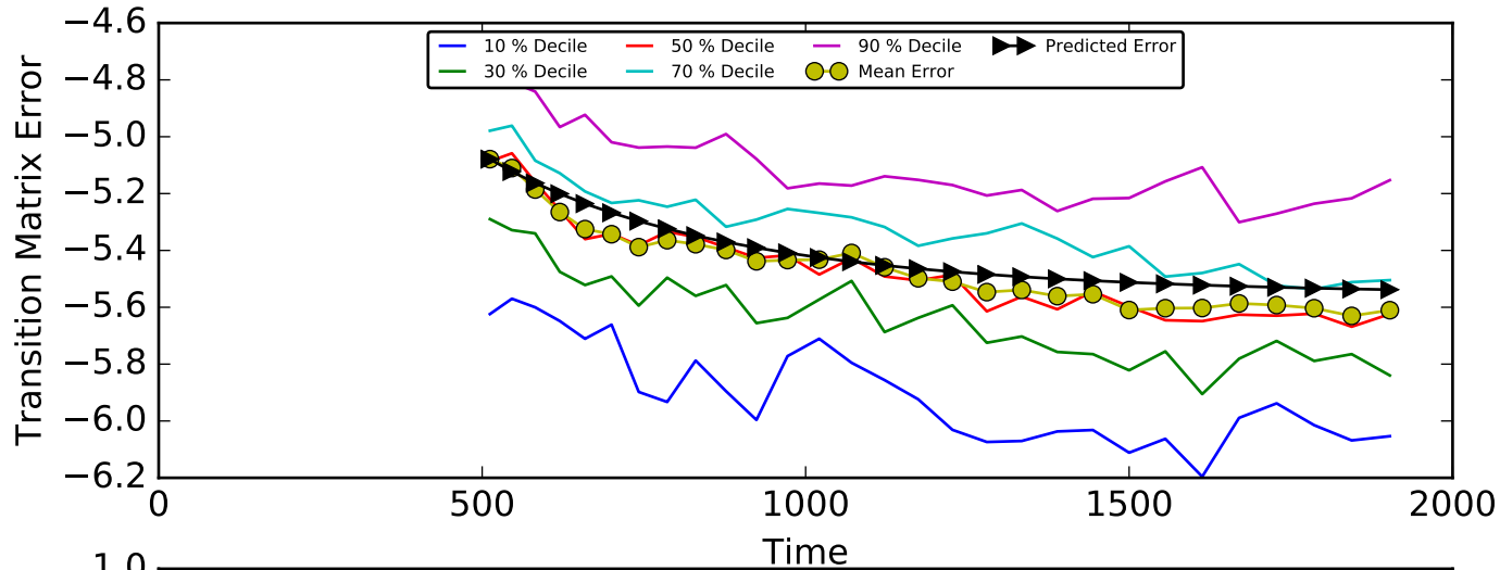
Distribution of Transition Matrix Error Along Trajectory (Bayes)
