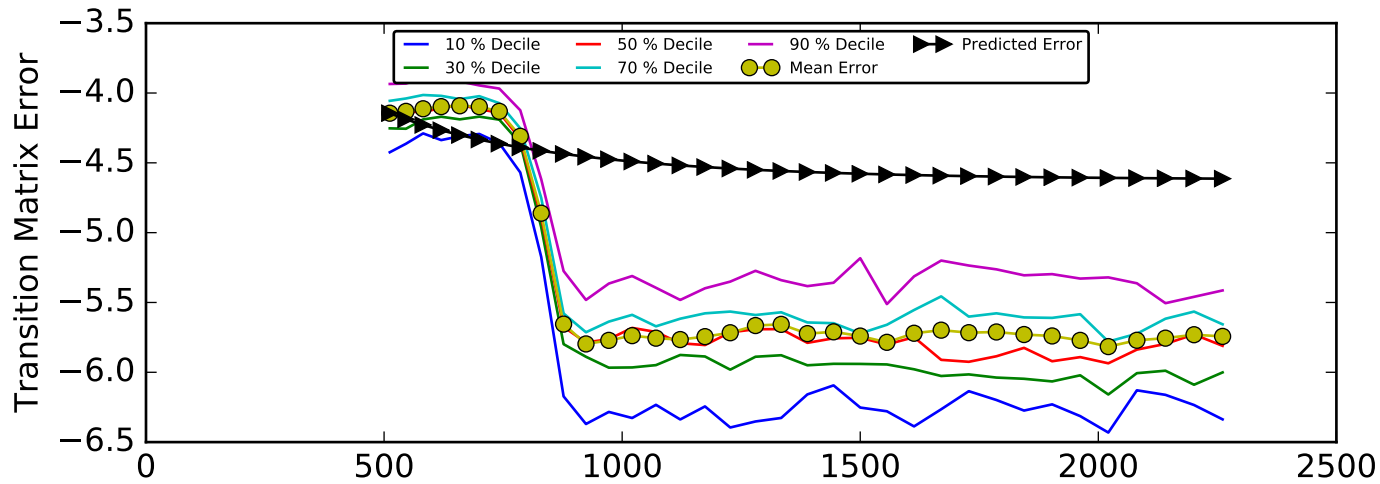
Distribution of Transition Matrix Error Along Trajectory (Bayes)
