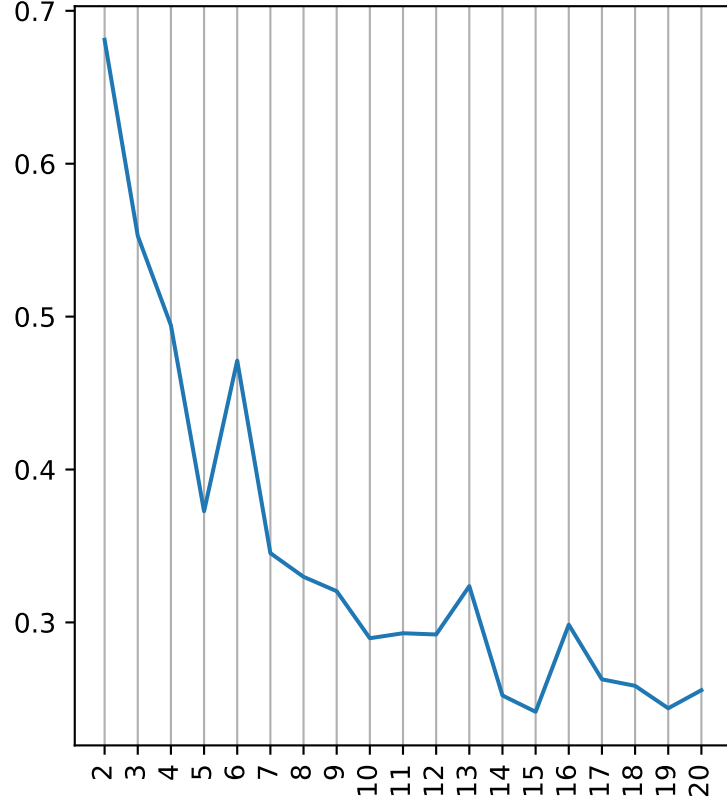
Silhouette_score
