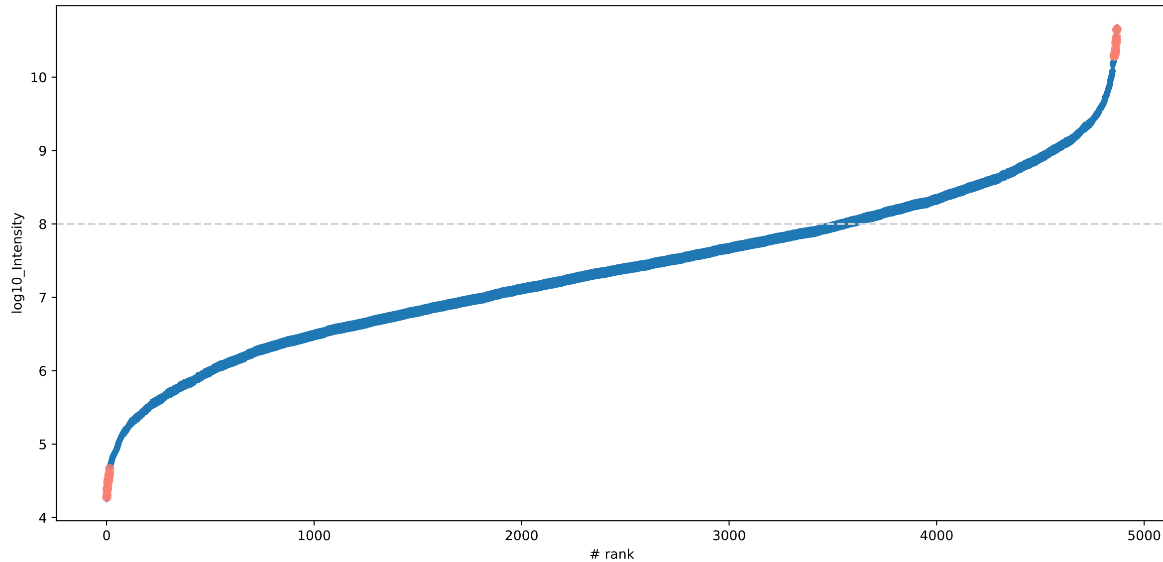
Rank Plot
