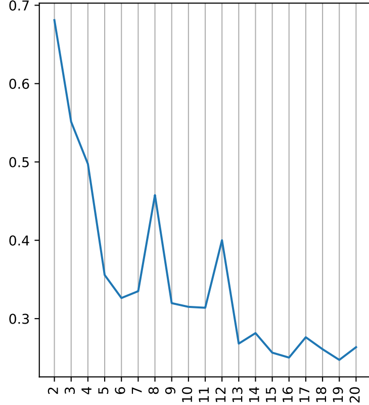
Silhouette_score
