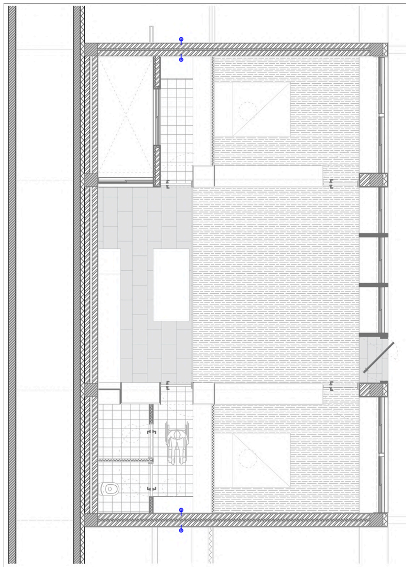
First drawing, housing complex on lower sector. Second and third drawings, example of house. That could be converted into commerce. Only one façade to the atmosphere facing south-east.
