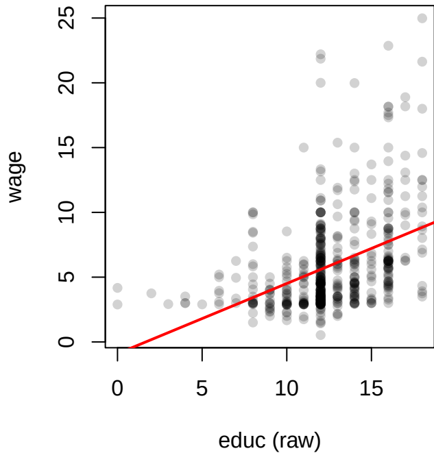
Simple regression view
