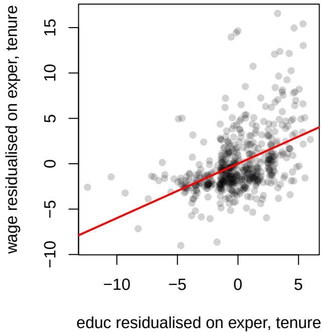
Partialling-out view (MLR slope)
