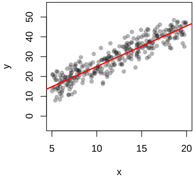
Homoskedastic: constant spread
