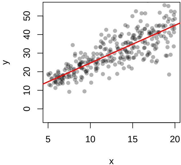
Heteroskedastic: fan-out spread
