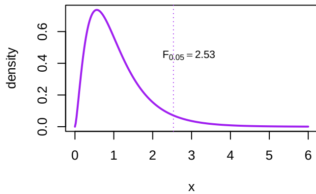
F with 5 and 30 df
