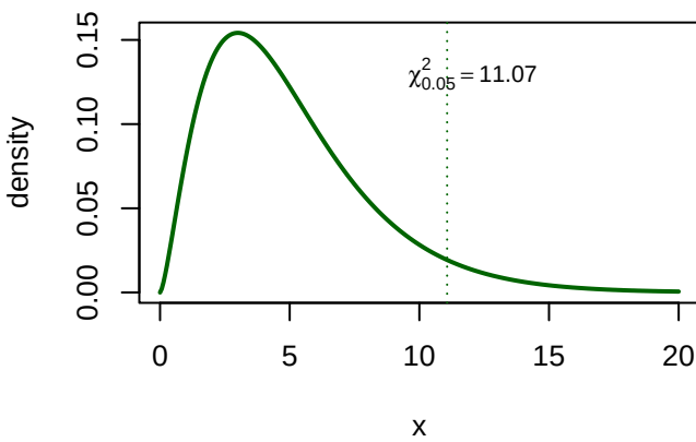
\chi^2 with 5 df
