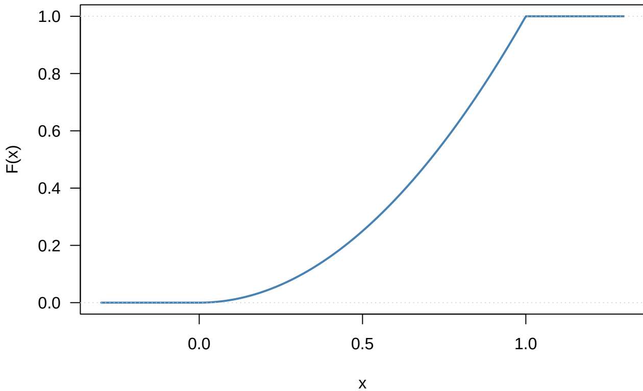
CDF: F(x) = x^2 on [0, 1]
