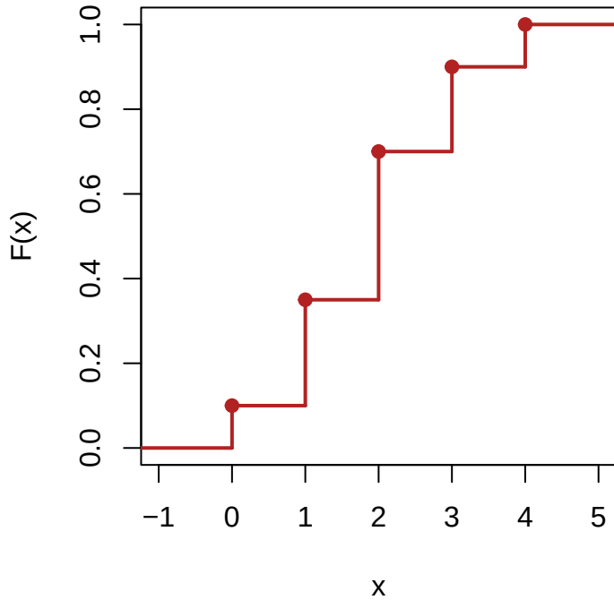
CDF
