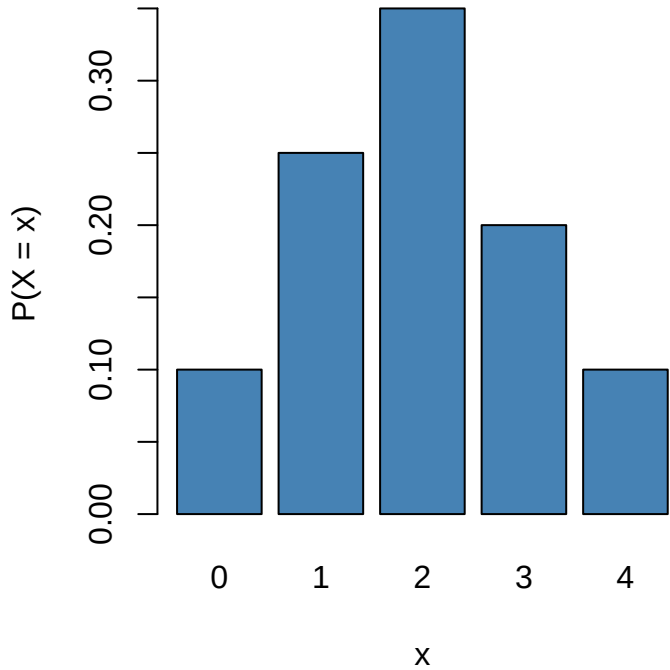
PMF
