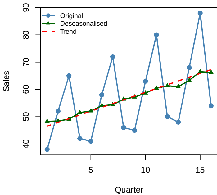
4. Original vs deseasonalised
