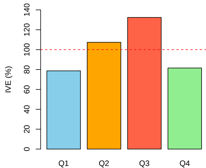
3. Seasonal indices
