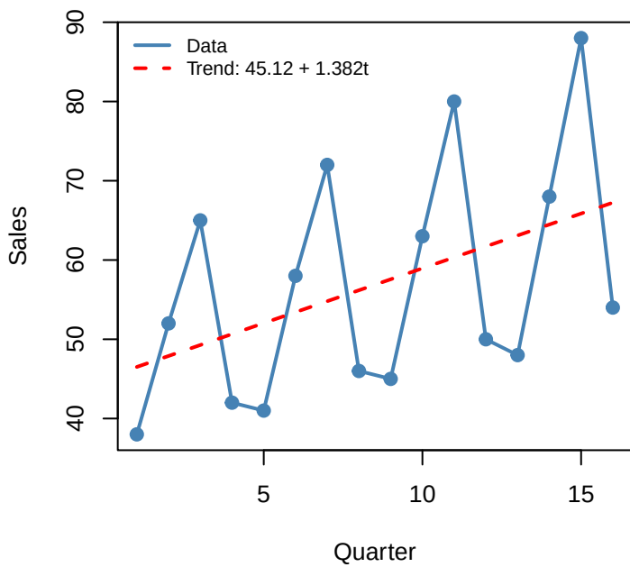
1. Original series
