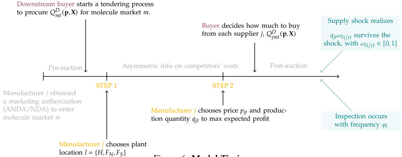
Figure 6: Model Timing
