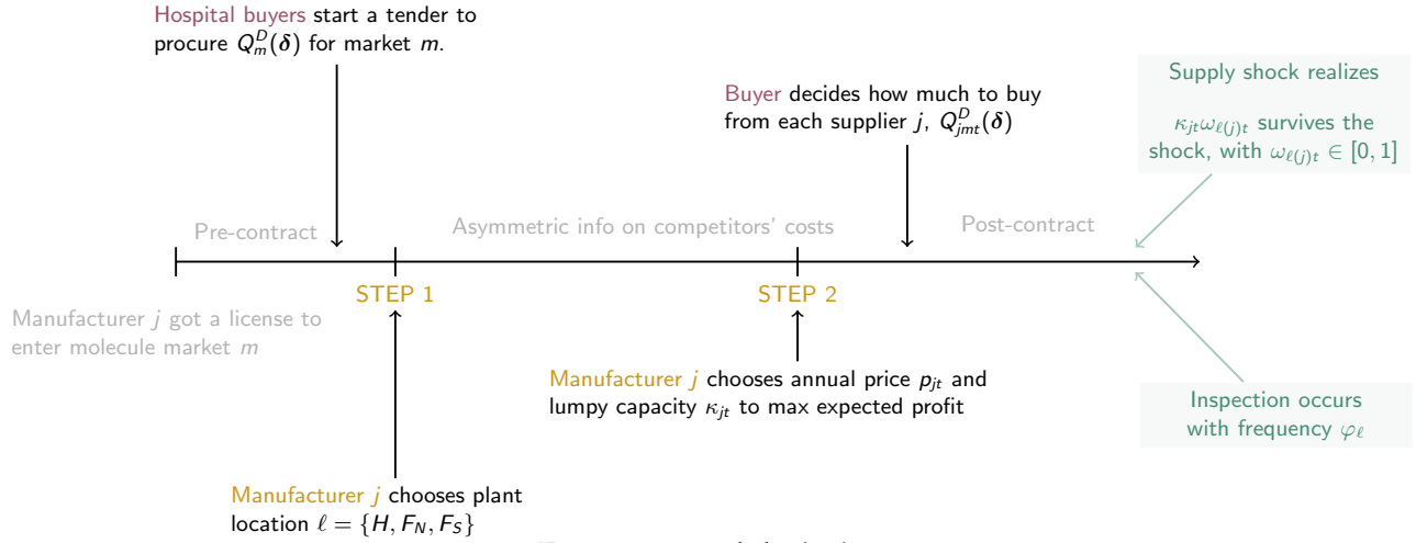
Figure 6: Model Timing
