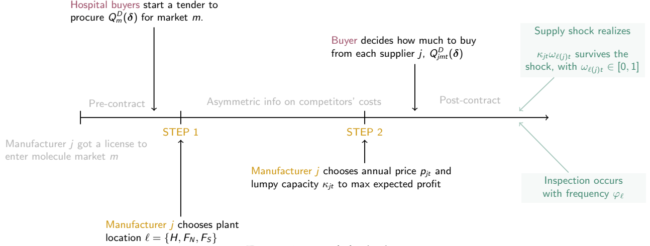
Figure 5: Model Timing
