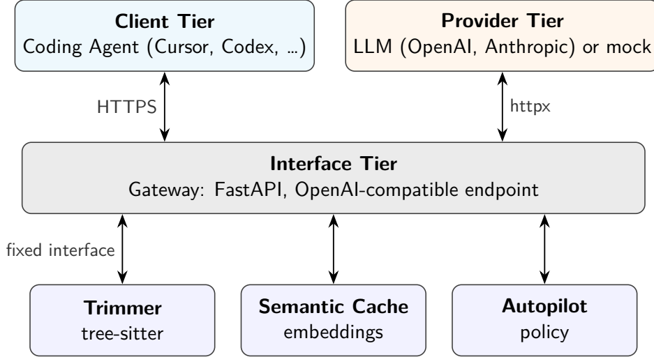
Figure 3: Three-tier architecture. The optimisation modules sit behind fixed interfaces, so each can be built and tested on its own.
