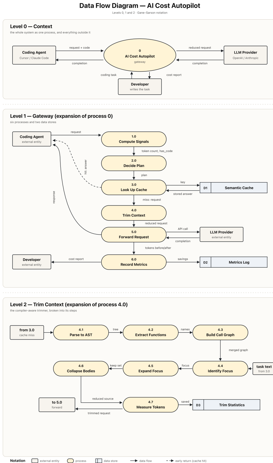
Figure 2.3: Data flow diagram, levels 0, 1 and 2.
