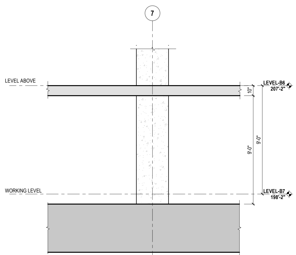
2 LEVEL-B7 BUILDING SECTION
