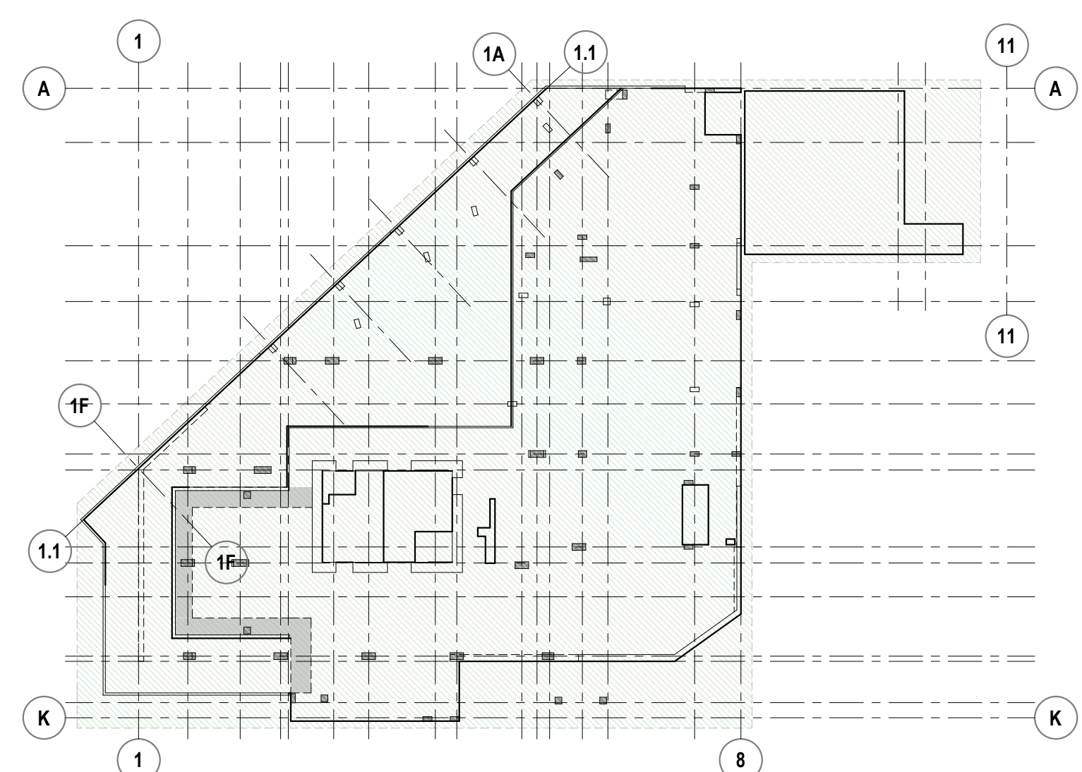
LEVEL-B2 KEY PLAN
