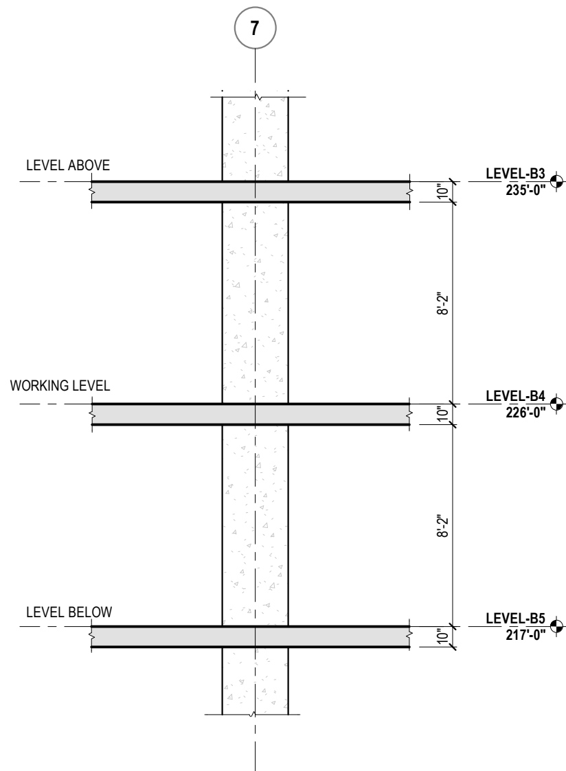
2 LEVEL-B4 BUILDING SECTION
