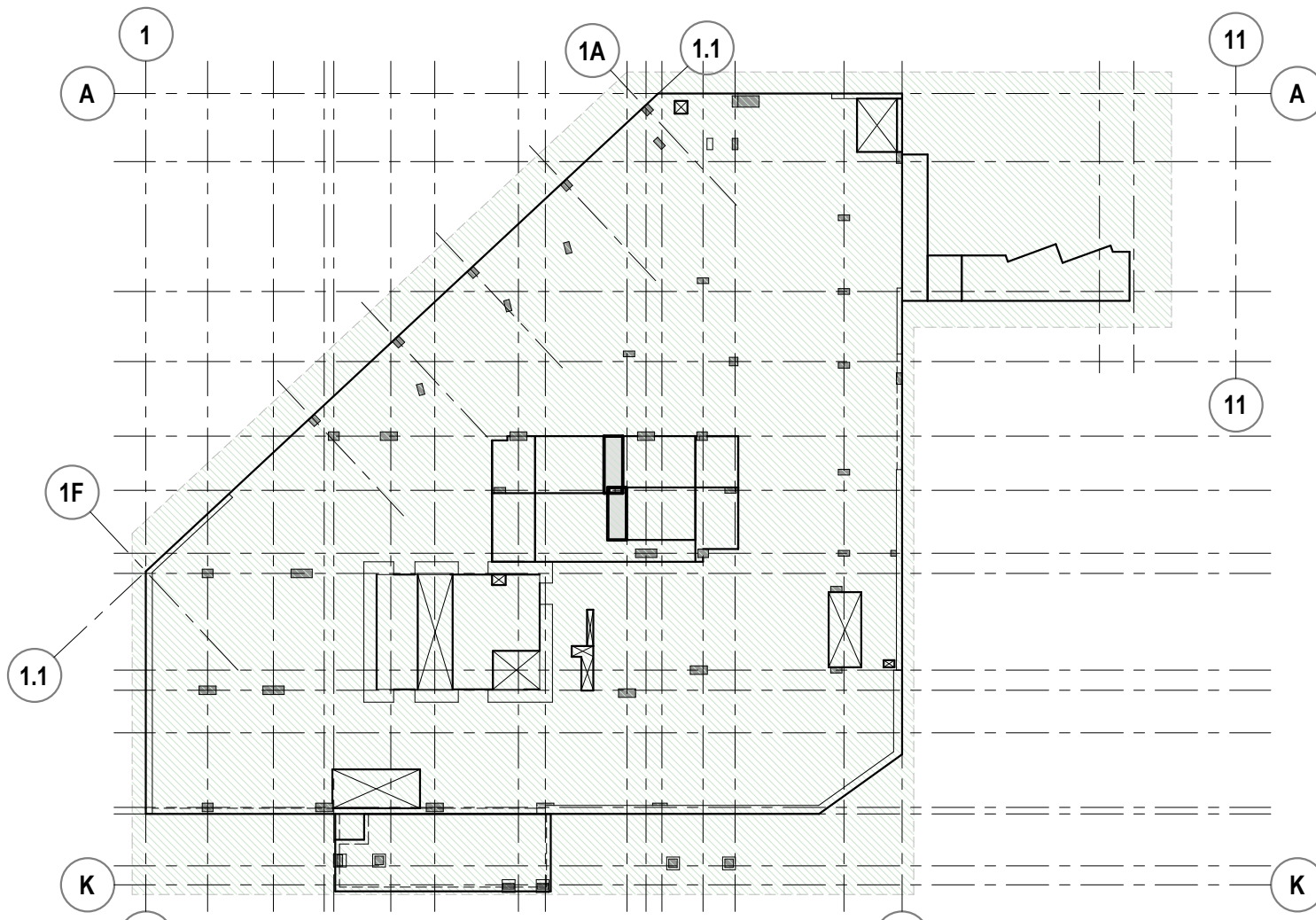
LEVEL-B4 KEY PLAN
