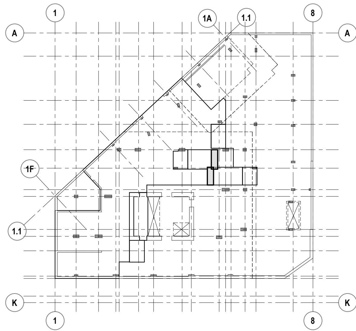
LEVEL-B7 KEY PLAN
