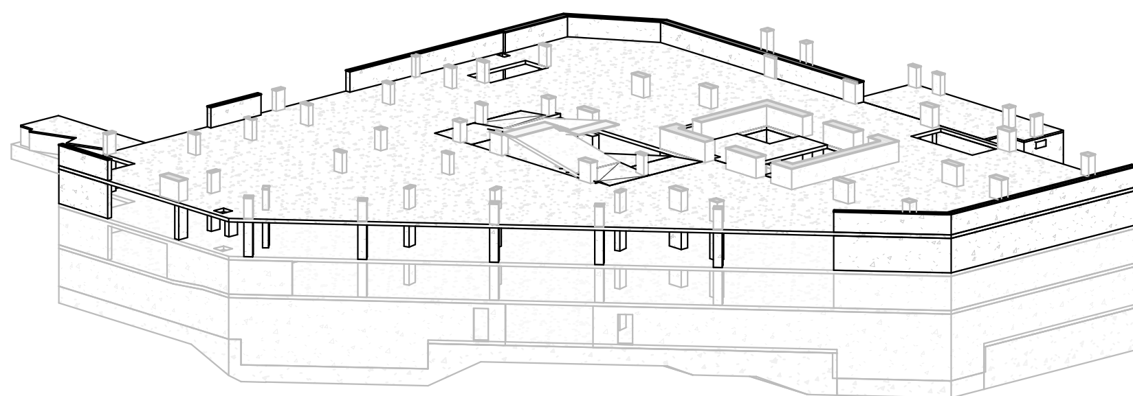
3D VIEW- LEVEL B4
