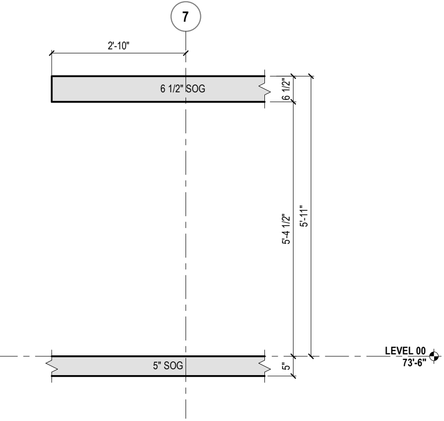
8 SLAB EDGE - MID LANDING REF: 1/11.0.0 1/2" = 1'-0"
