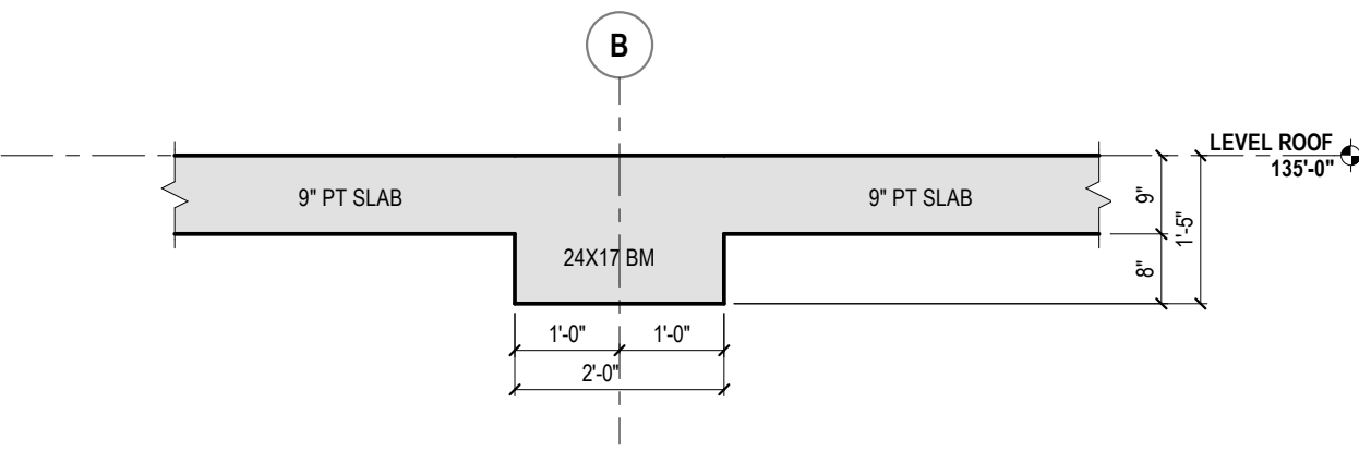
1 24"x17" BEAM AT ROOF LEVEL REF: 1/11.4.0 1/2" = 1'-0"
