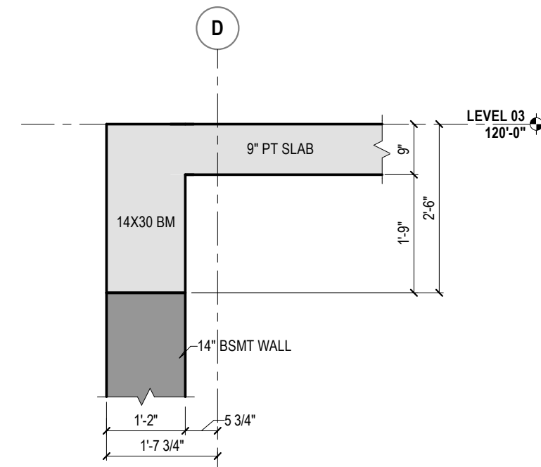
7 14"x30" BEAM AT WALL REF: 1/1/130 1/2" = 1'-0"
