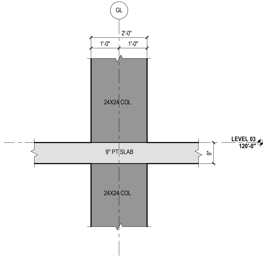
5 24"x24" COLUMN AT LEVEL 03 REF: 1/11.3.0 1/2" = 1'-0"
