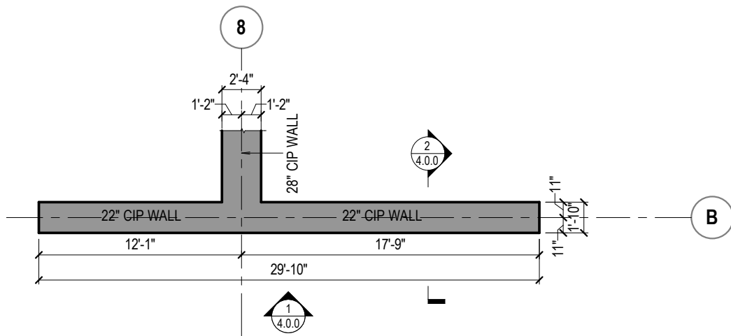
3 PLAN VIEW - SHEAR WALL ELEVATION GL B 1/8" = 1'-0"
