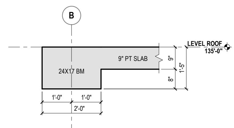
2 24"x17" BEAM AT ROOF REF: 1/11.4.0 1/2" = 1'-0"
