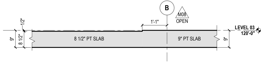
11 1/2" SLAB DEPRESSION REF: 1/1/130 1/2" = 1'-0"
