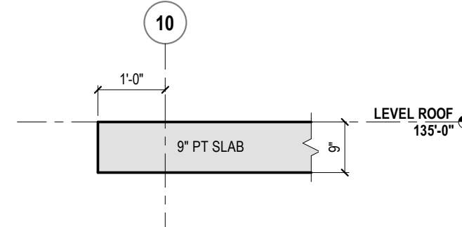
4 EDGE OF SLAB GL 10 REF: 1/11.4.0 1/2" = 1'-0"
