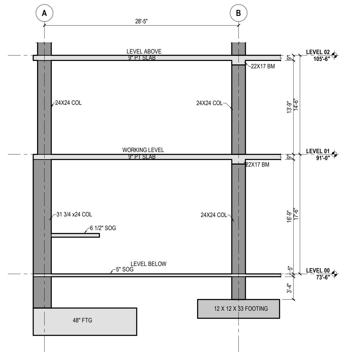
2 BUILDING ELEVATION - LEVEL 01
