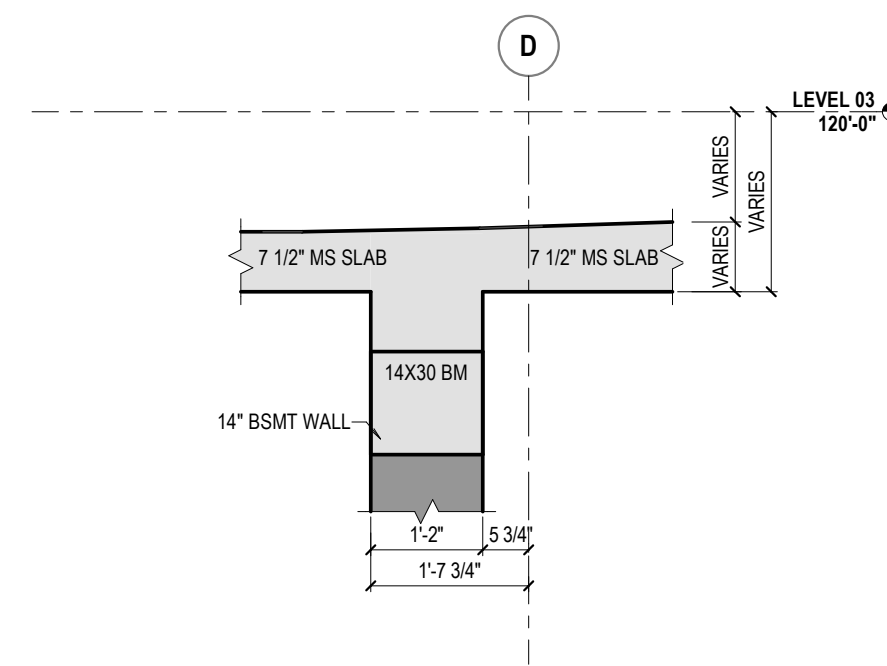
8 MILD REINFORCED BEAT AT BSMT WALL REF: 1/1/130 1/2" = 1'-0"
