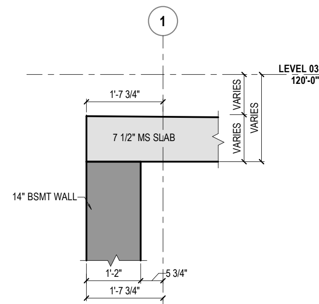
6 MILD-REINFORCED SLAB AT SIDEWALK INTRFACE REF: 1/1/130 1/2" = 1'-0"
