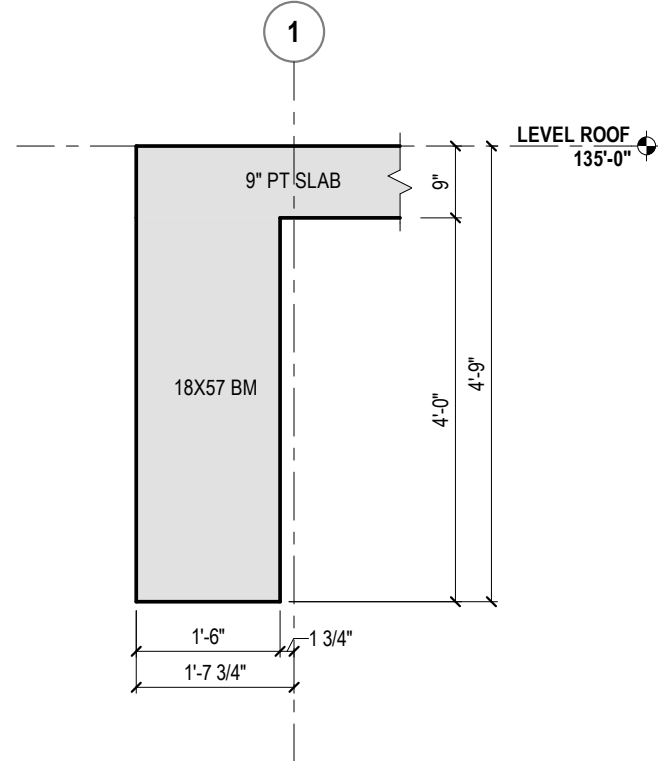
7 18x57 BM AT ROOF REF: 1/11.4.0 1/2" = 1'-0"
