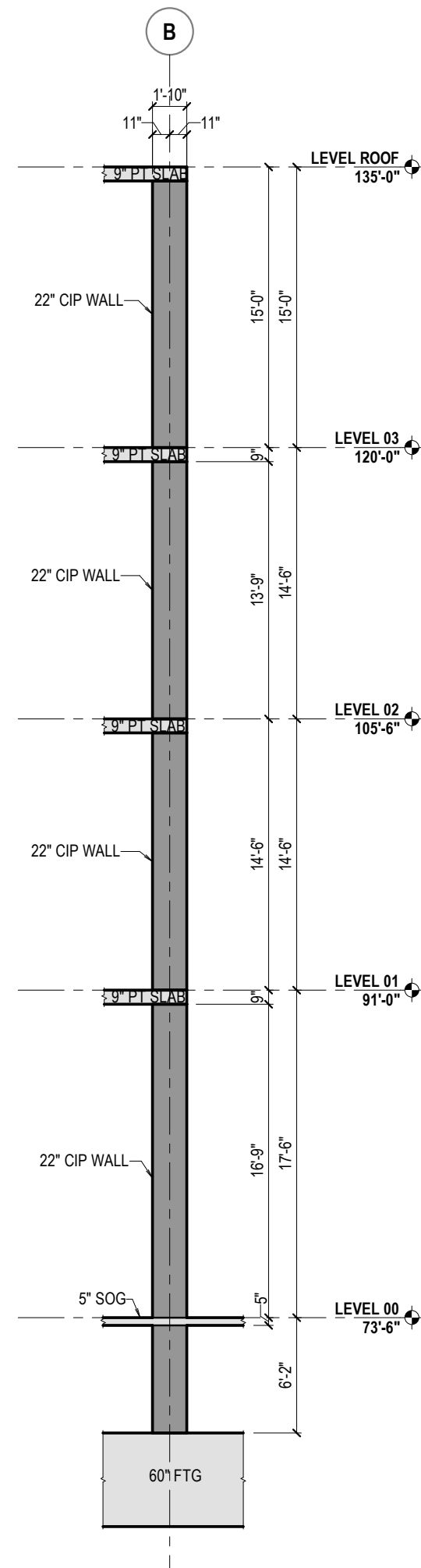
2 WALL SECTION - SHEAR WALL ELEVATION GL B 1/8" = 1'-0"
