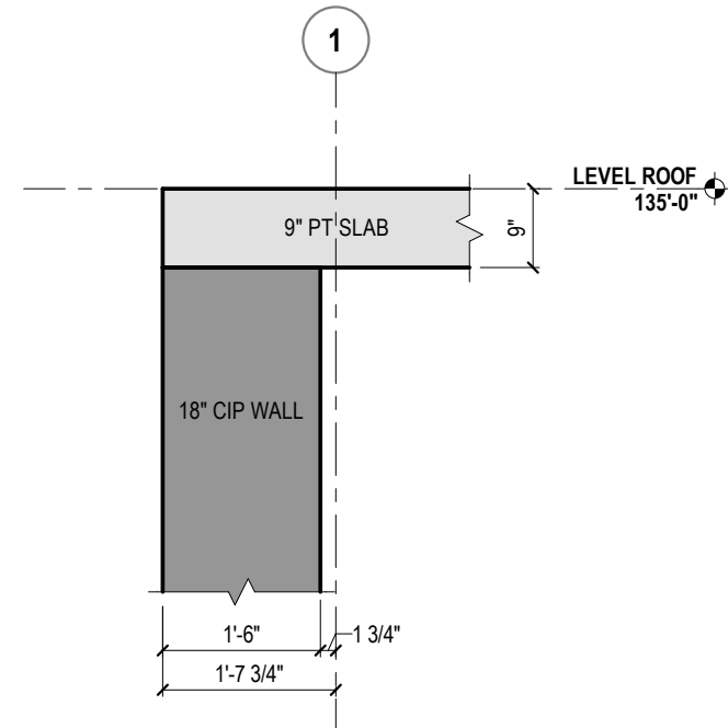
14 EOS LEVEL ROOF REF: 1/1/140 1/2" = 1'-0"
