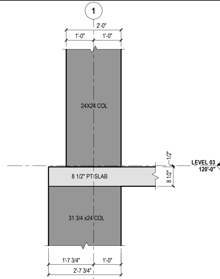
5 COLUMN TRANSITION REF: 1/1/130 1/2" = 1'-0"
