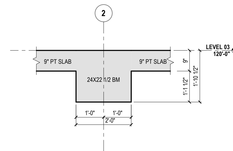
4 24"x22 1/2" BEAM AT LEVEL 03 REF: 1/1/130 1/2" = 1'-0"
