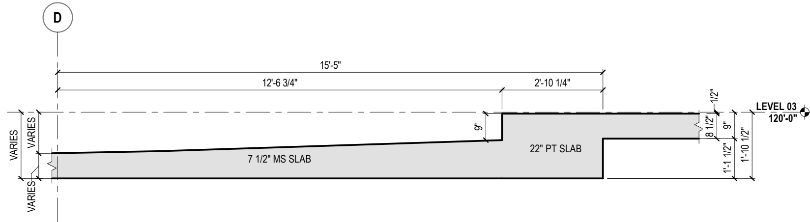
9 THICKENED SLAB AT SLAB STEP REF: 1/1/130 3/8" = 1'-0"
