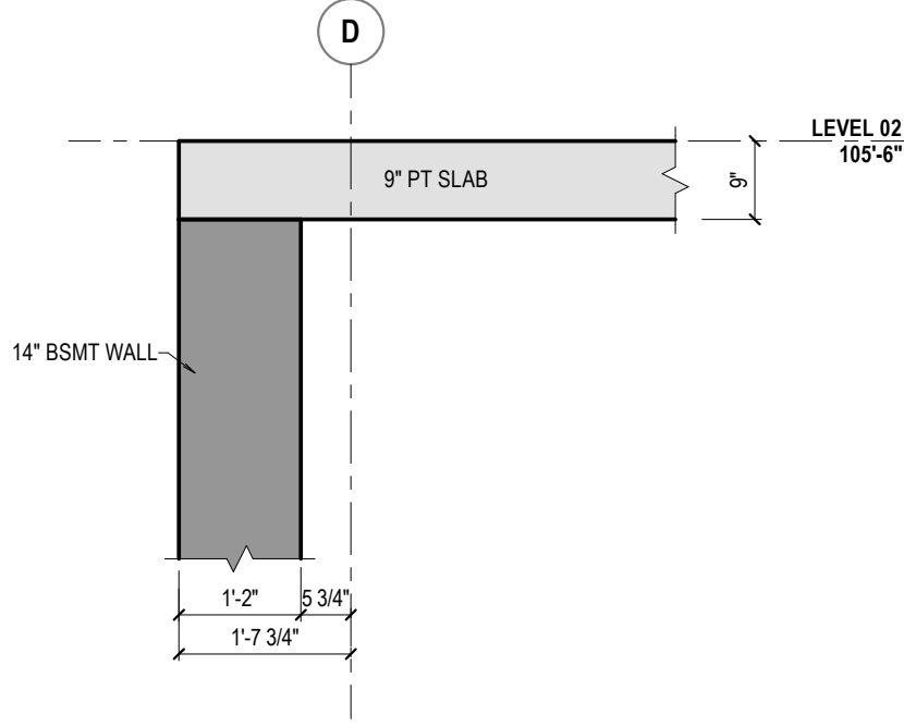
6 BSMNT WALL AT EOS LEVEL 02 REF: 1/11.2.0 1/2" = 1'-0"
