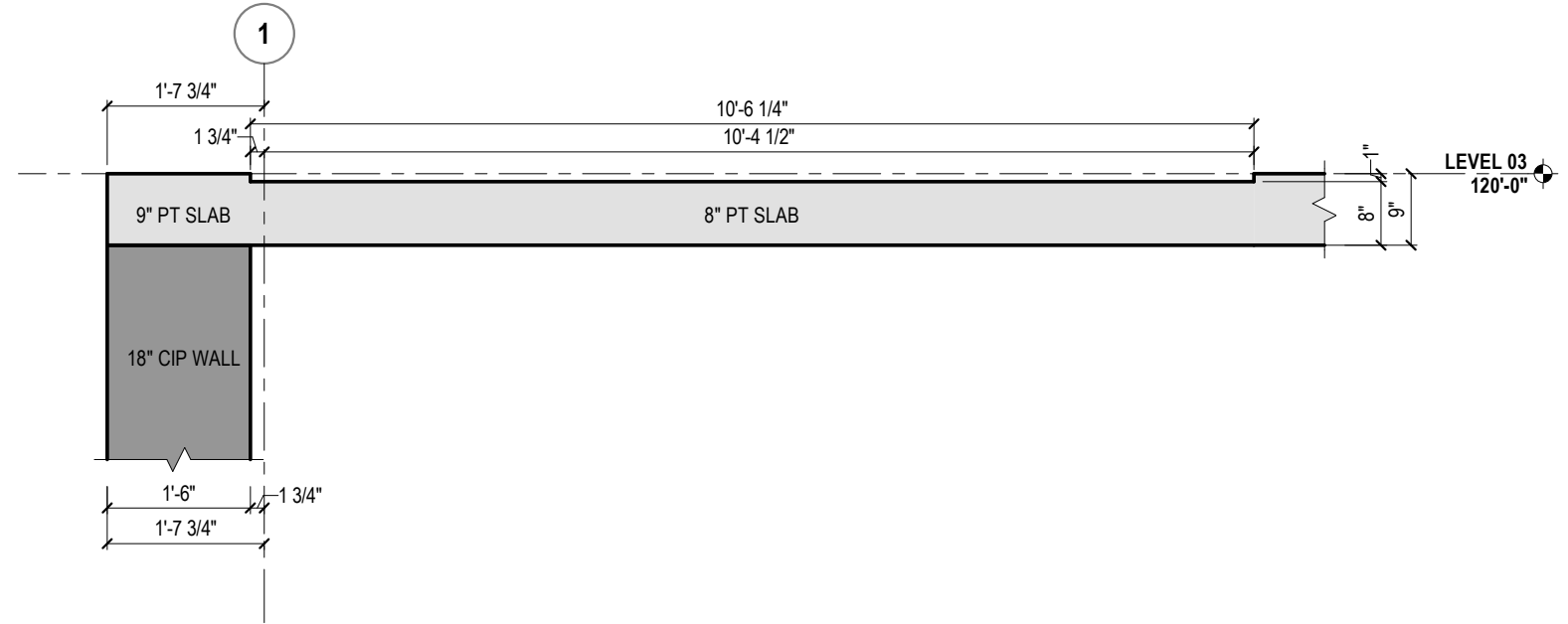
10 1" SLAB DEPRESSION AT EOS REF: 1/1/130 1/2" = 1'-0"
