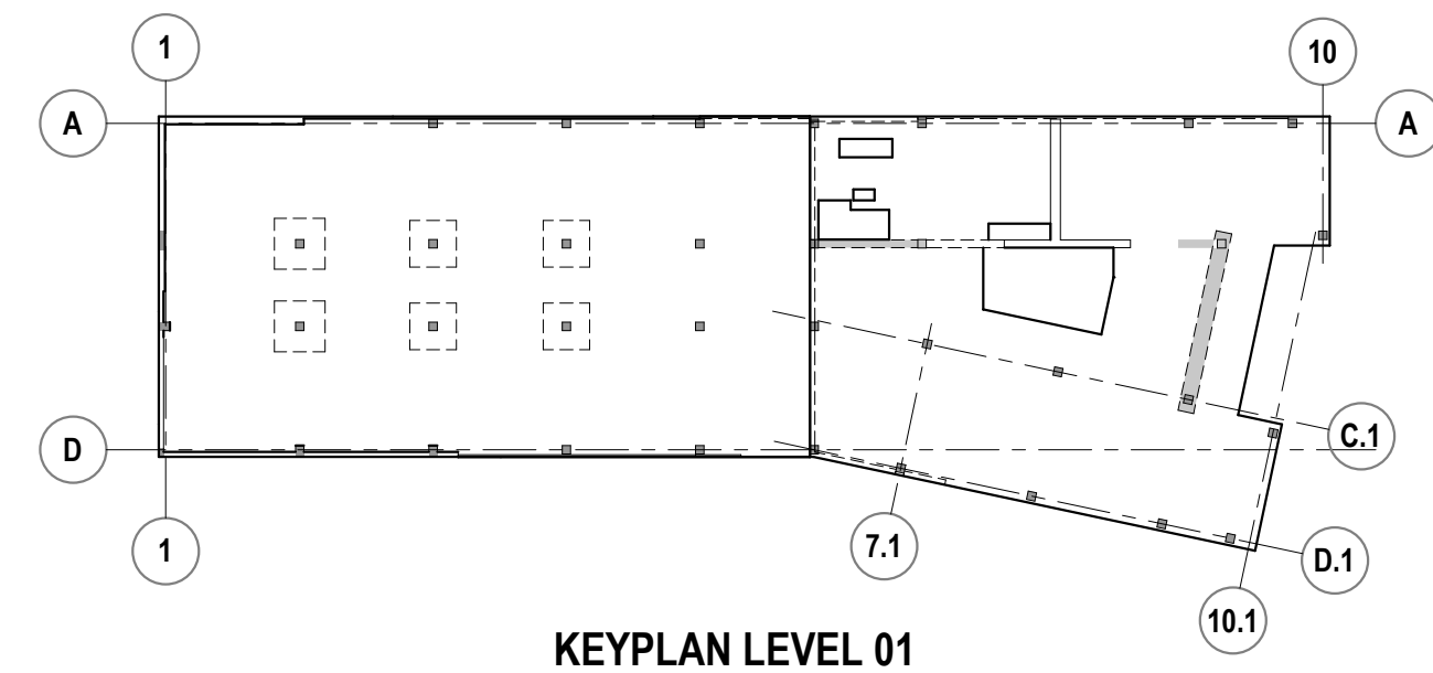
KEYPLAN LEVEL 01
