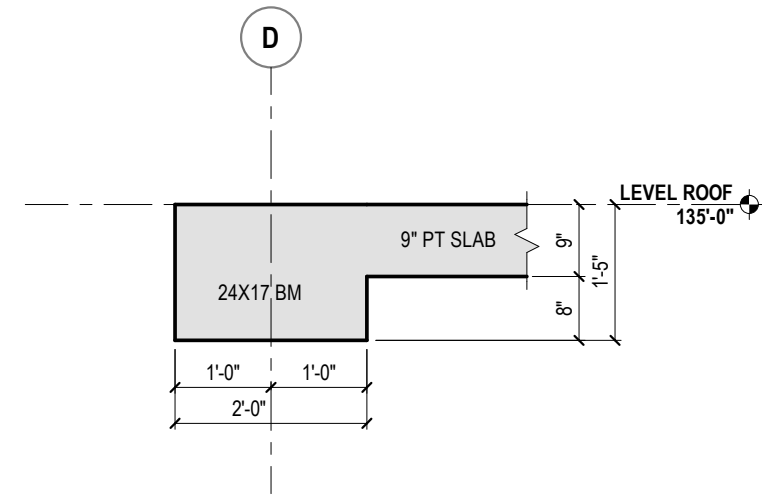
13 24"x17" BEAM AT EDGE REF: 1/1/140 1/2" = 1'-0"
