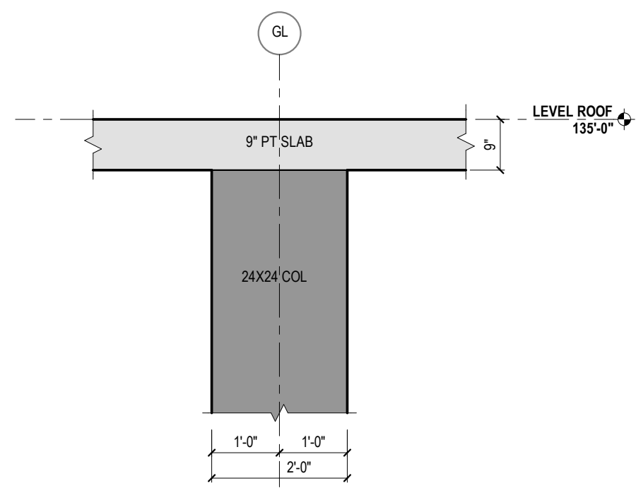
3 24"x24" COLUMN AT ROOF REF: 1/11.4.0 1/2" = 1'-0"
