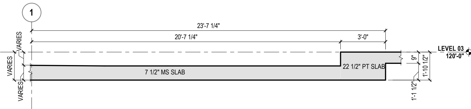
12 TICKENED SLAB AT SLAB STEP LEVEL 03 REF: 1/1/130 1/4" = 1'-0"
