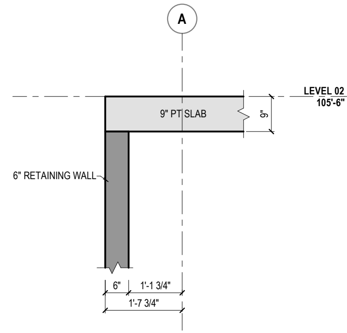
1 EOS AT RETAINING WALL LEVEL 02 REF: 1/1/120 1/2" = 1'-0"
