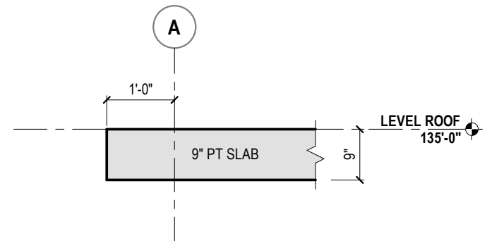
15 SLAB EDGE AT ROOF LEVEL REF: 1/1/140 1/2" = 1'-0"
