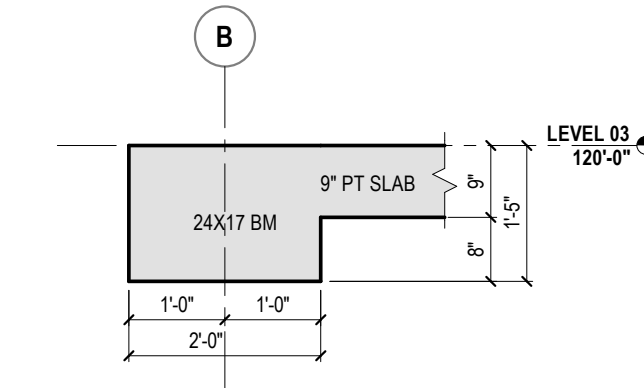
3 24"x17" BEAM LEVEL 03 REF: 1/1/130 1/2" = 1'-0"
