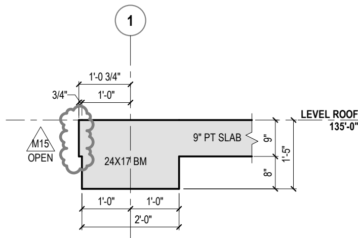
16 24"x17" BEAM AT EOS - ROOF REF: 1/1/140 1/2" = 1'-0"
