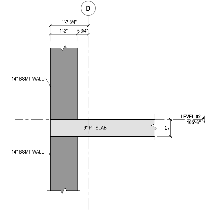
2 EOS AT BSMT WALL REF: 1/1/120 1/2" = 1'-0"
