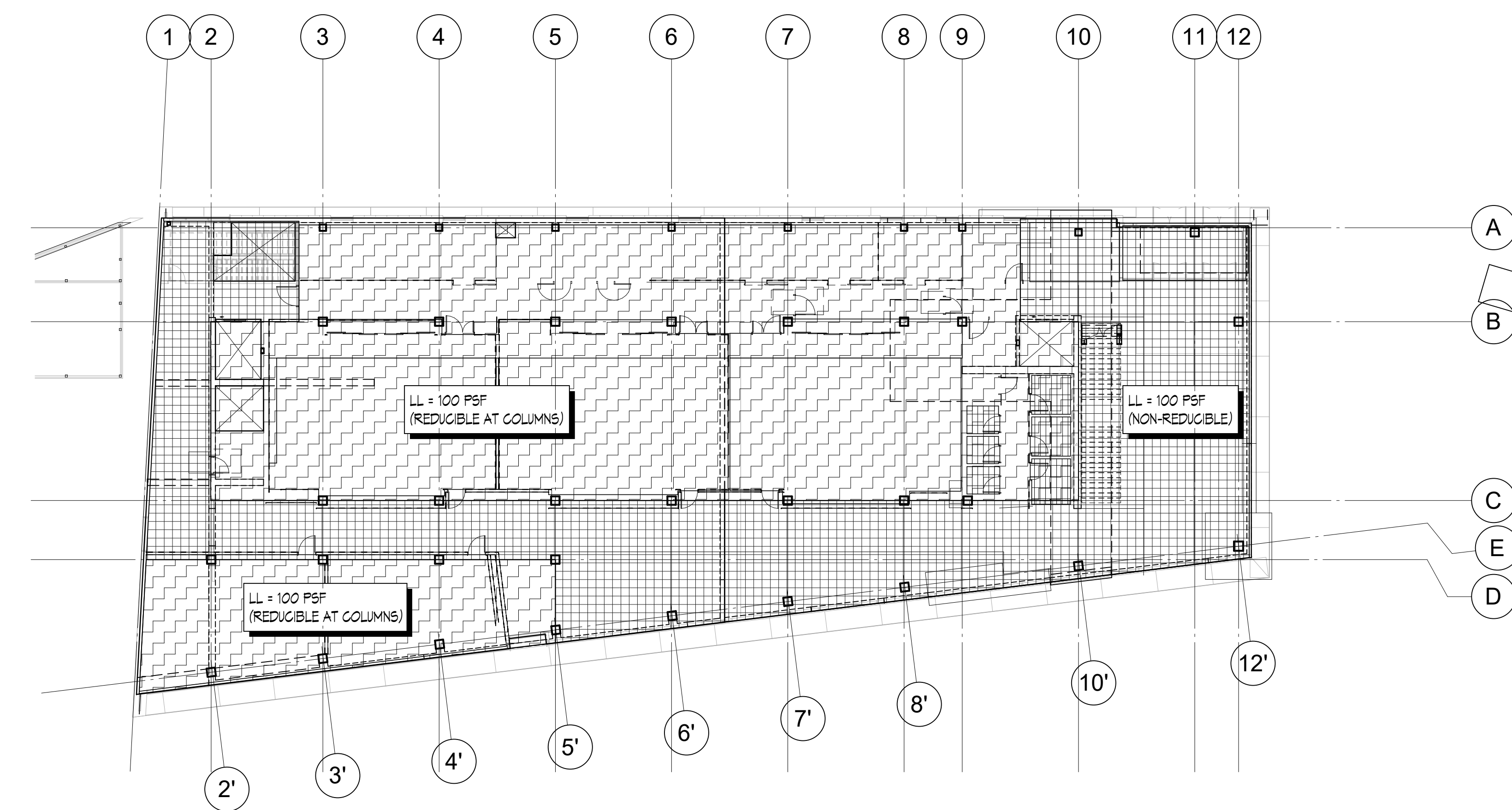
4 LEVEL 2 - LIVE LOAD 1/16" = 1'-0"
