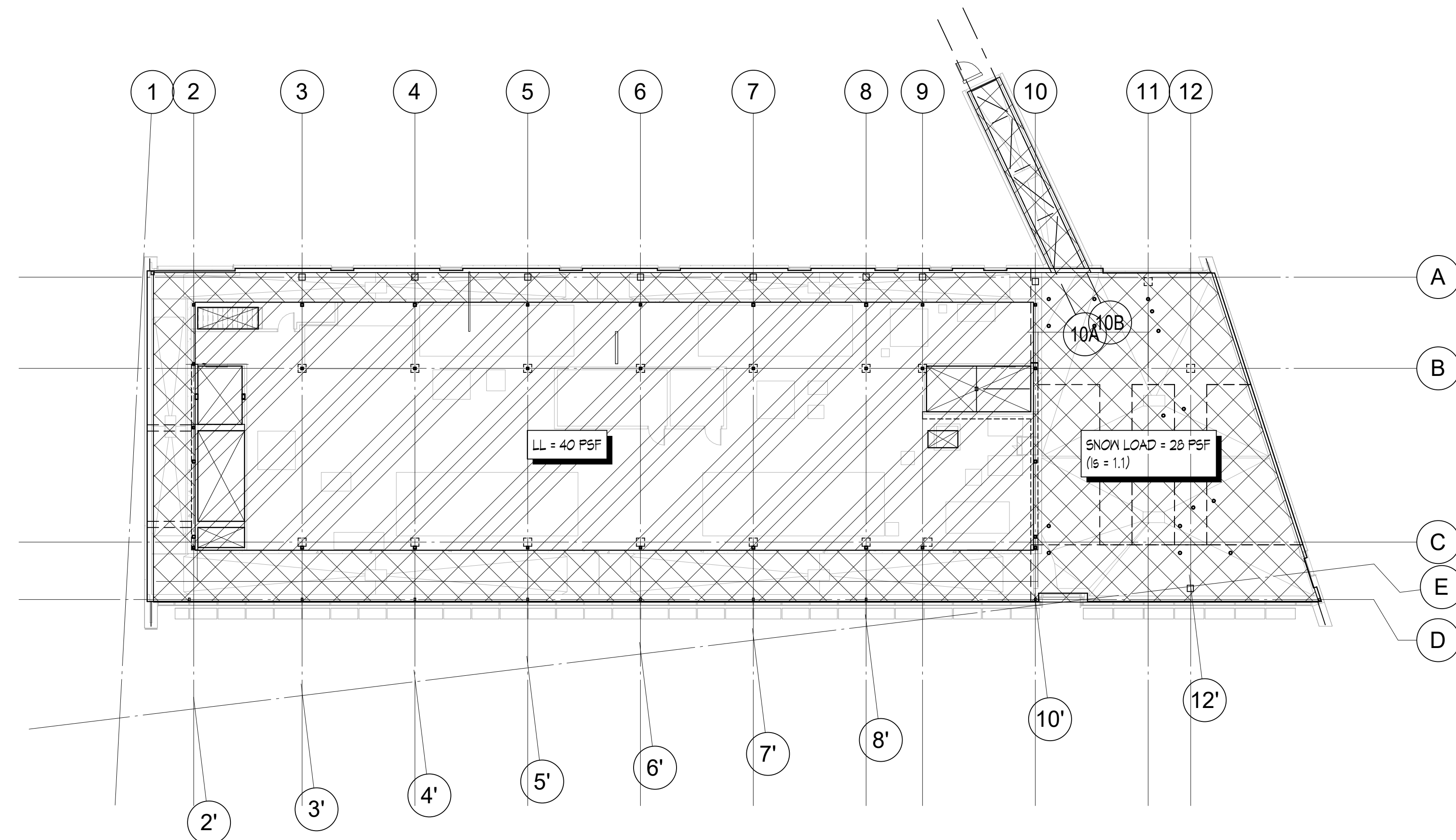
2 LEVEL 4 - LIVE LOAD 1/16" = 1'-0"
