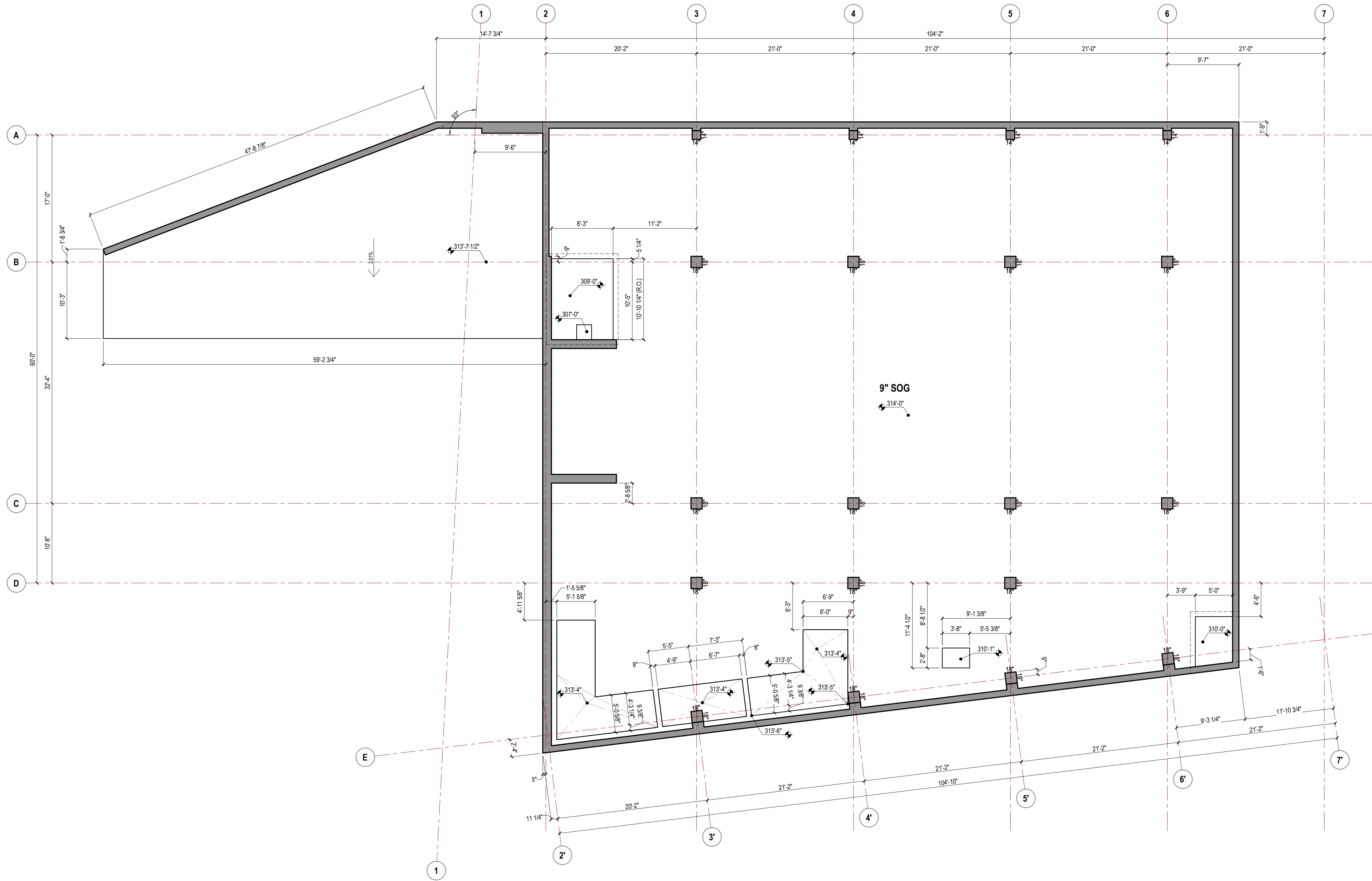
1 LEVEL-1 SLAB ON GRADE FLOOR PLAN REF: 311.10 1/8" = 1'-0"
