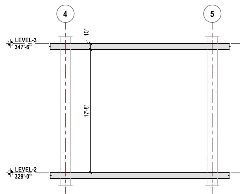
3 BUILDING SECTION 1/8" = 1'-0"
