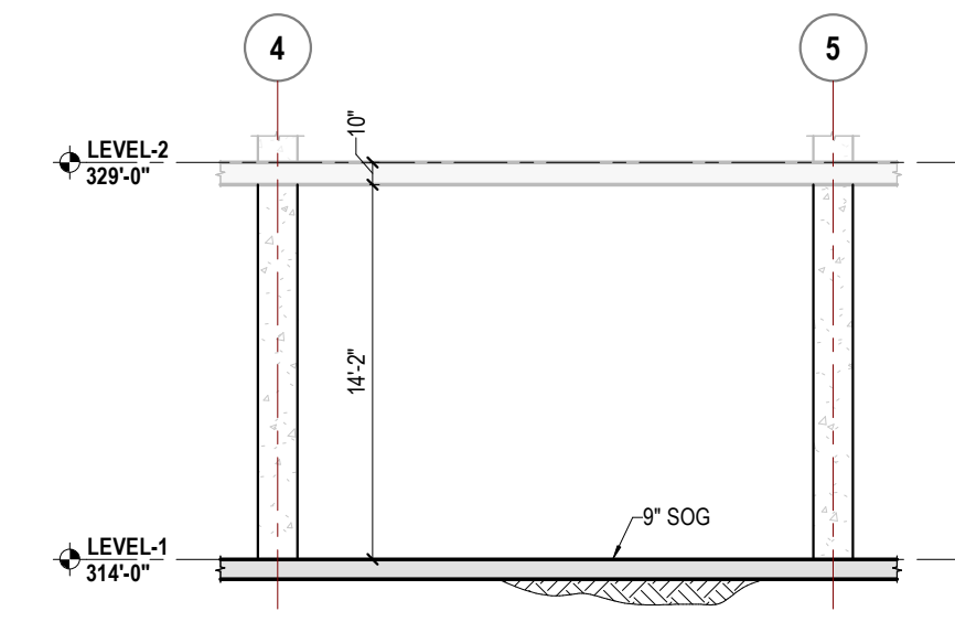
3 BUILDING SECTION 1/8" = 1'-0"
