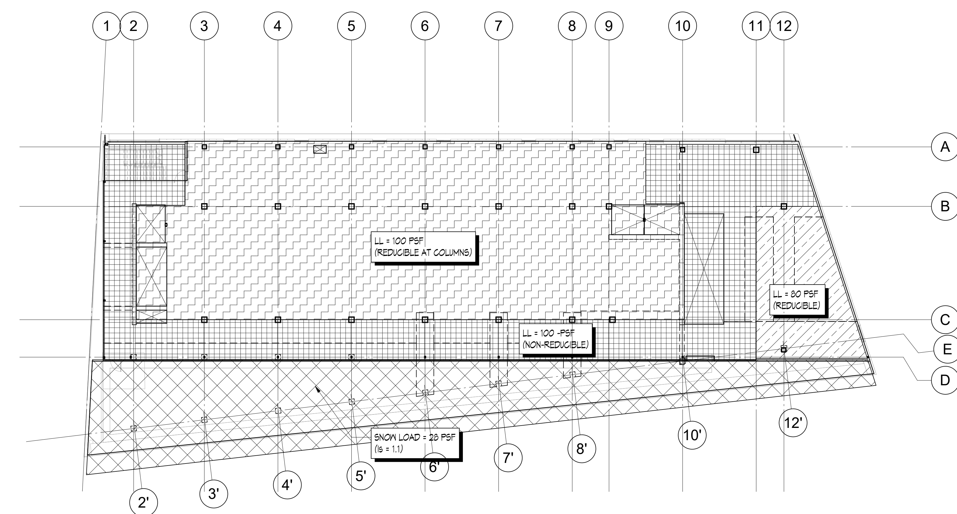
6 LEVEL 3 - LIVE LOAD 1/16" = 1'-0" |
