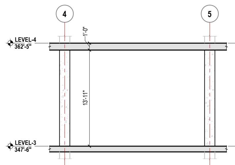
3 BUILDING SECTION 1/8" = 1'-0"
