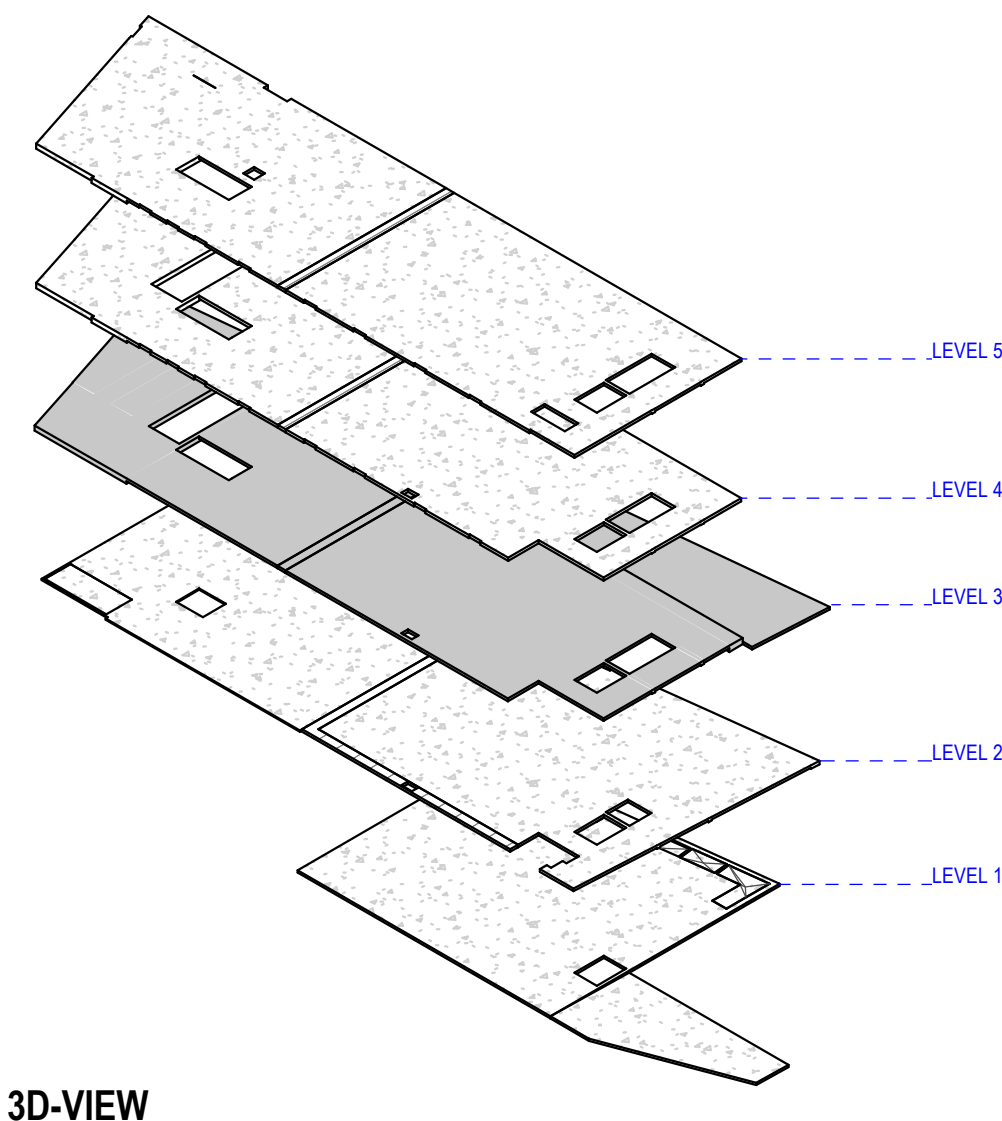
2 3D-VIEW
