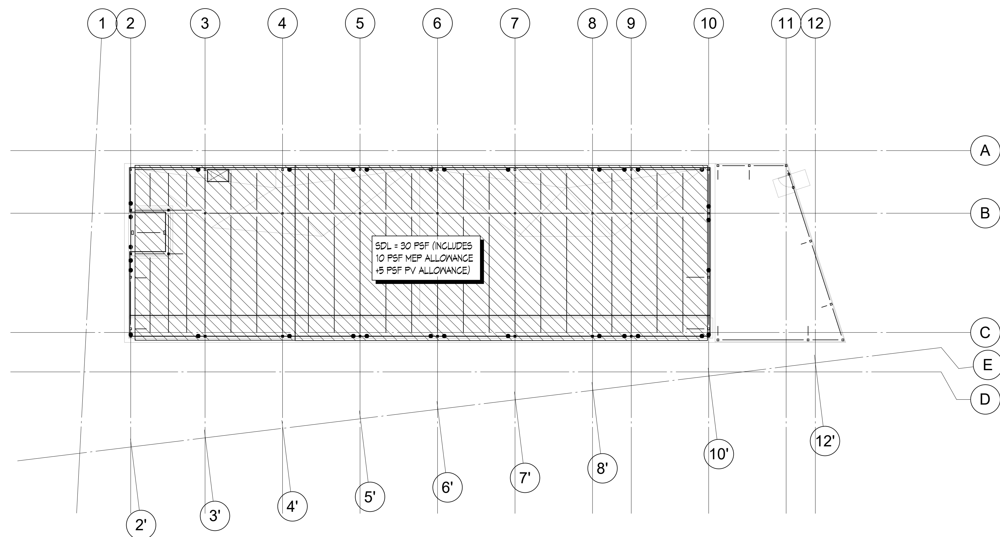
5 ROOF - SUPERIMPOSED DEAD LOAD 1/16" = 1'-0"
