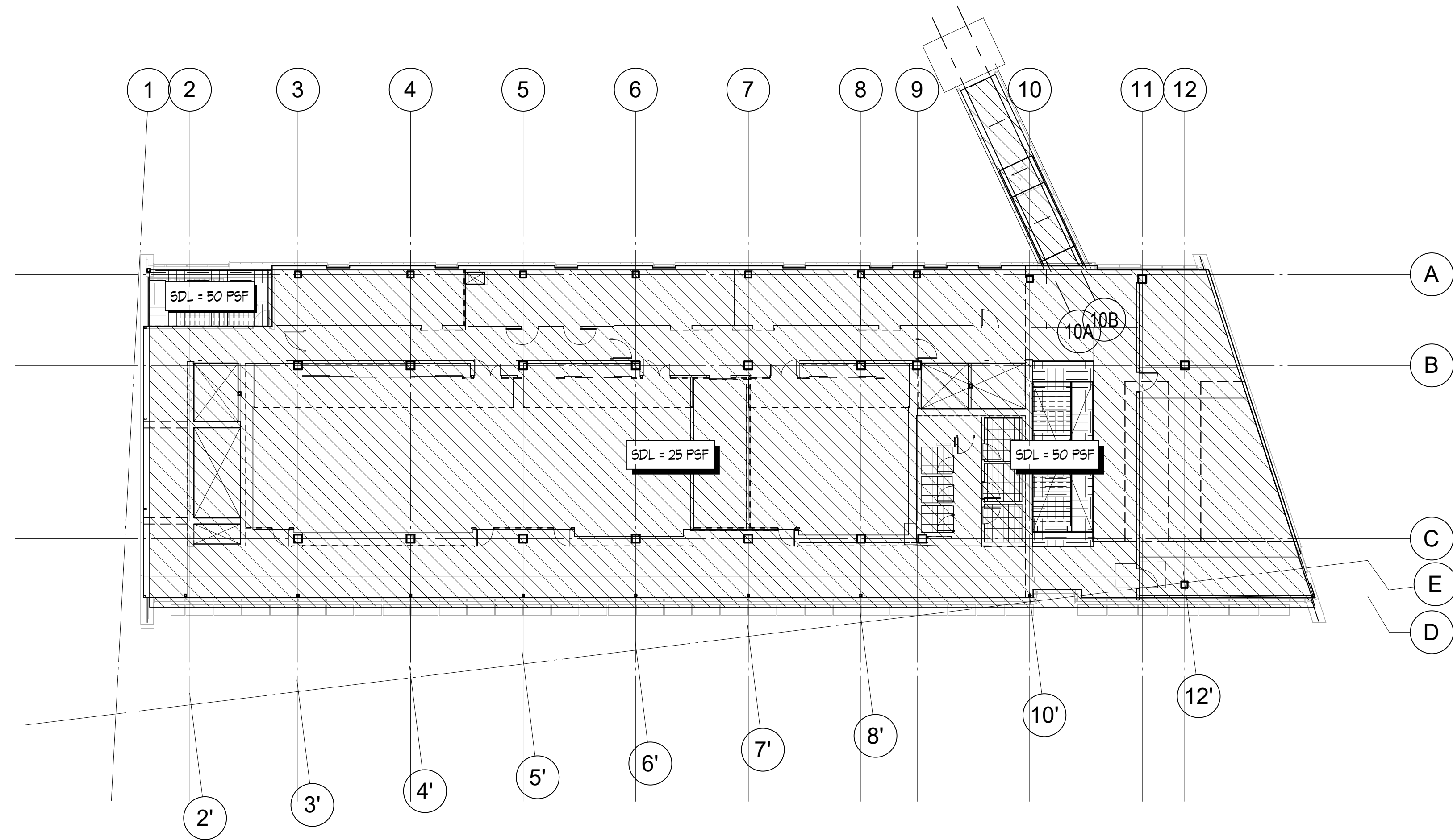
1 LEVEL 4 - SUPERIMPOSED DEAD LOAD 1/16" = 1'-0"
