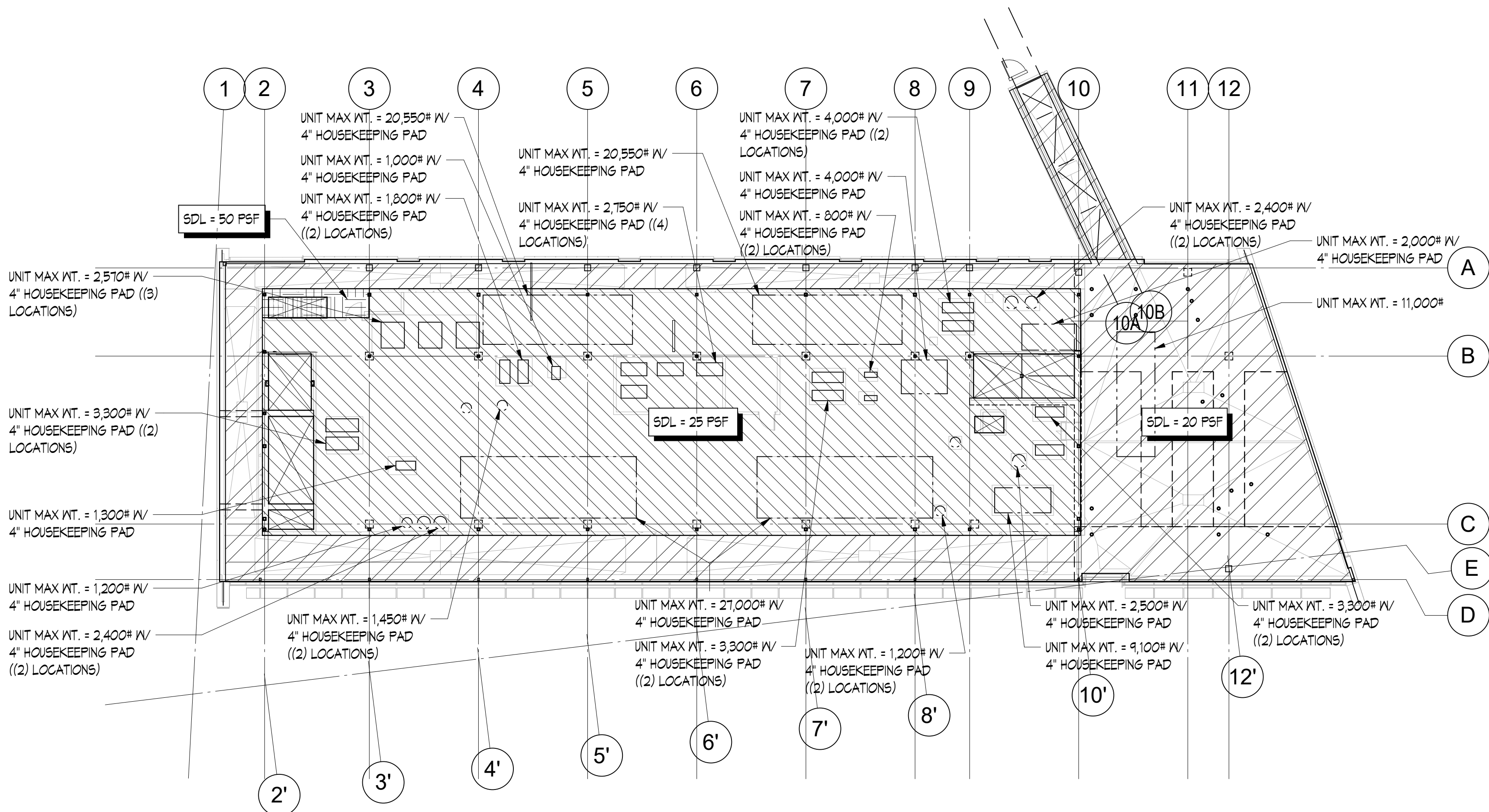
1 LEVEL 4 - SUPERIMPOSED DEAD LOAD 1/16" = 1'-0"
