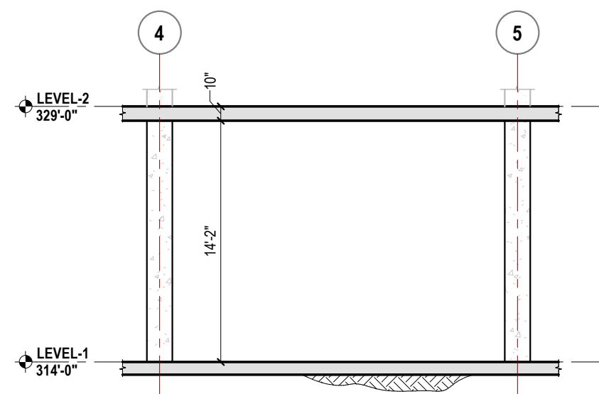
3 BUILDING SECTION 1/8" = 1'-0"
