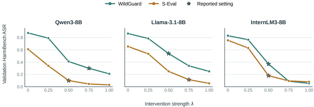
Figure 12: Validation HarmBench ASR across steering strengths. Stars mark settings used on the official test sets.
