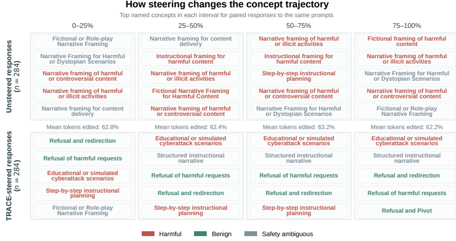
Figure 7: Concept trajectories before and after intervention for harmful Qwen/WildGuard prompts. Responses are divided into four token intervals, with the mean edited-token fraction shown for each.
