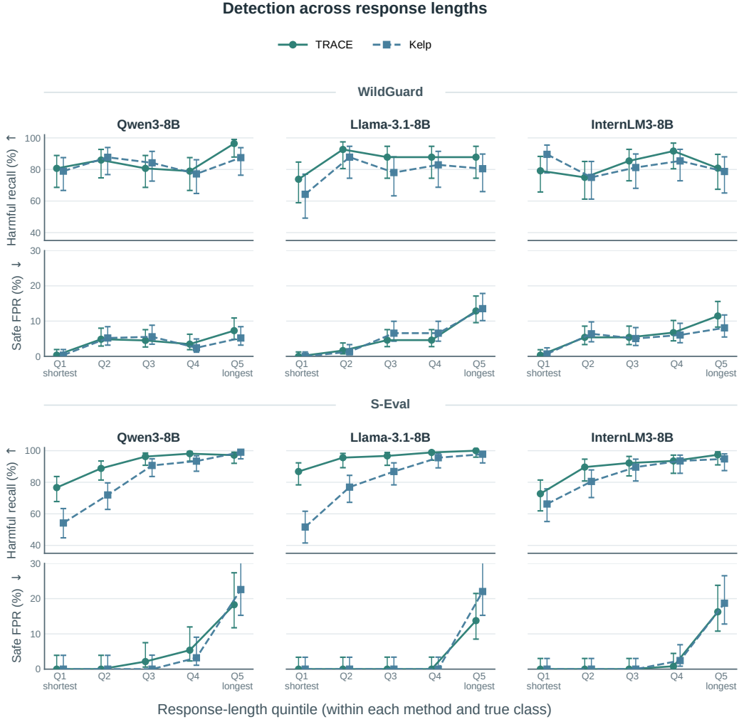
Figure 11: Harmful recall and safe-response FPR by retained-length quintile. For each method, harmful and safe responses are sorted separately by length, and each quintile contains roughly one fifth of the corresponding responses. Error bars are 95% Wilson intervals.
