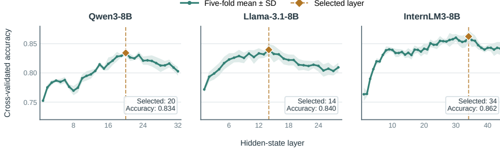
Figure 3: Five-fold WildGuard probe accuracy by read layer. Diamonds mark the selected layers.
