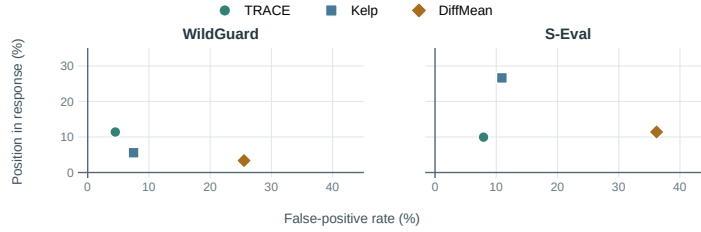
Figure 2: Qwen3-8B median first-detection position and FPR at each method’s reported threshold.
