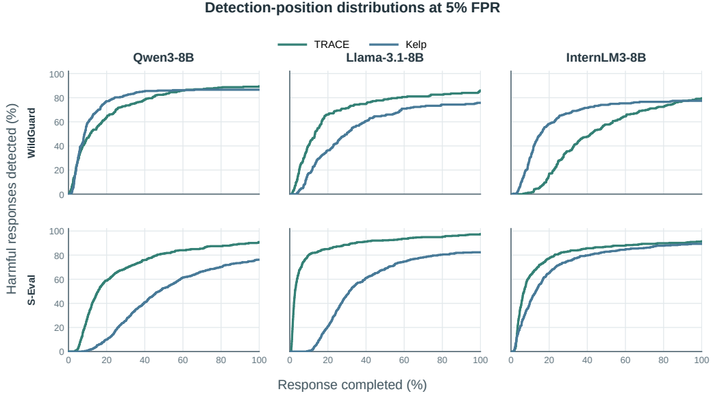
Figure 10: Cumulative first-detection coverage at thresholds selected for a 5% validation FPR. Rows are datasets and columns are generators.
