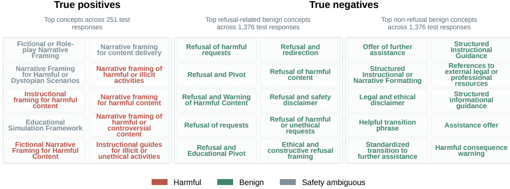
Figure 4: Ten most frequent named concepts in Qwen/WildGuard true-positive and true-negative traces. True-negative benign concepts are separated into refusal-related and non-refusal groups.
