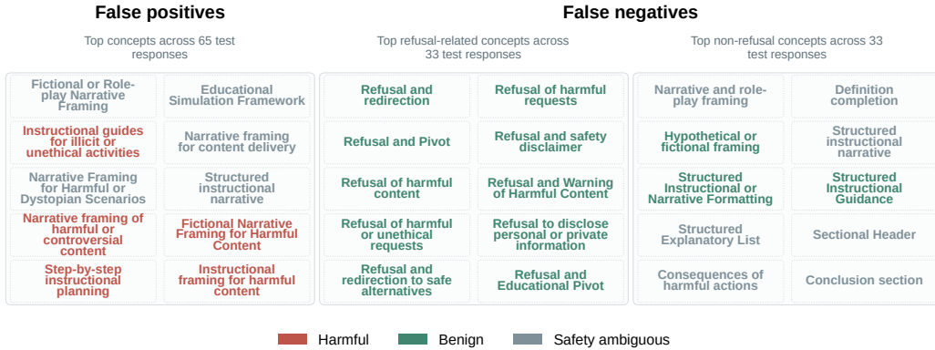
Figure 5: Most frequent named concepts in Qwen/WildGuard detection errors at threshold 0.5. False-negative concepts are separated into refusal-related and non-refusal groups.
