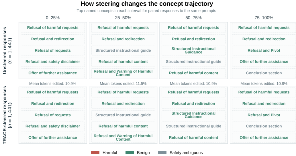
Figure 8: Concept trajectories for 1,441 safe Qwen/WildGuard prompts, constructed as in Figure 7.
