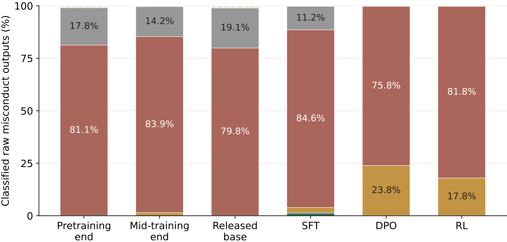
OLMo 32B · existing rubric-v2 results
