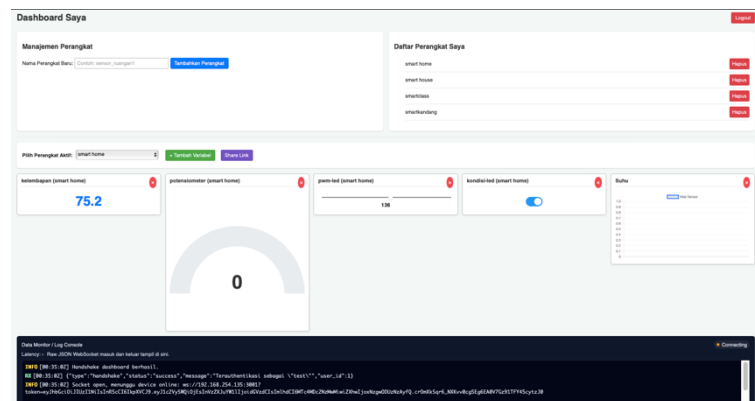
Gambar 5. UI/UX Dashboard Platform UNIOT
