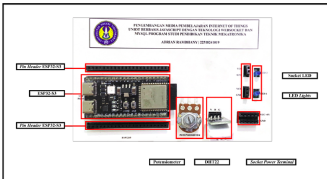
Gambar 6. Trainer Kit UNIOT
