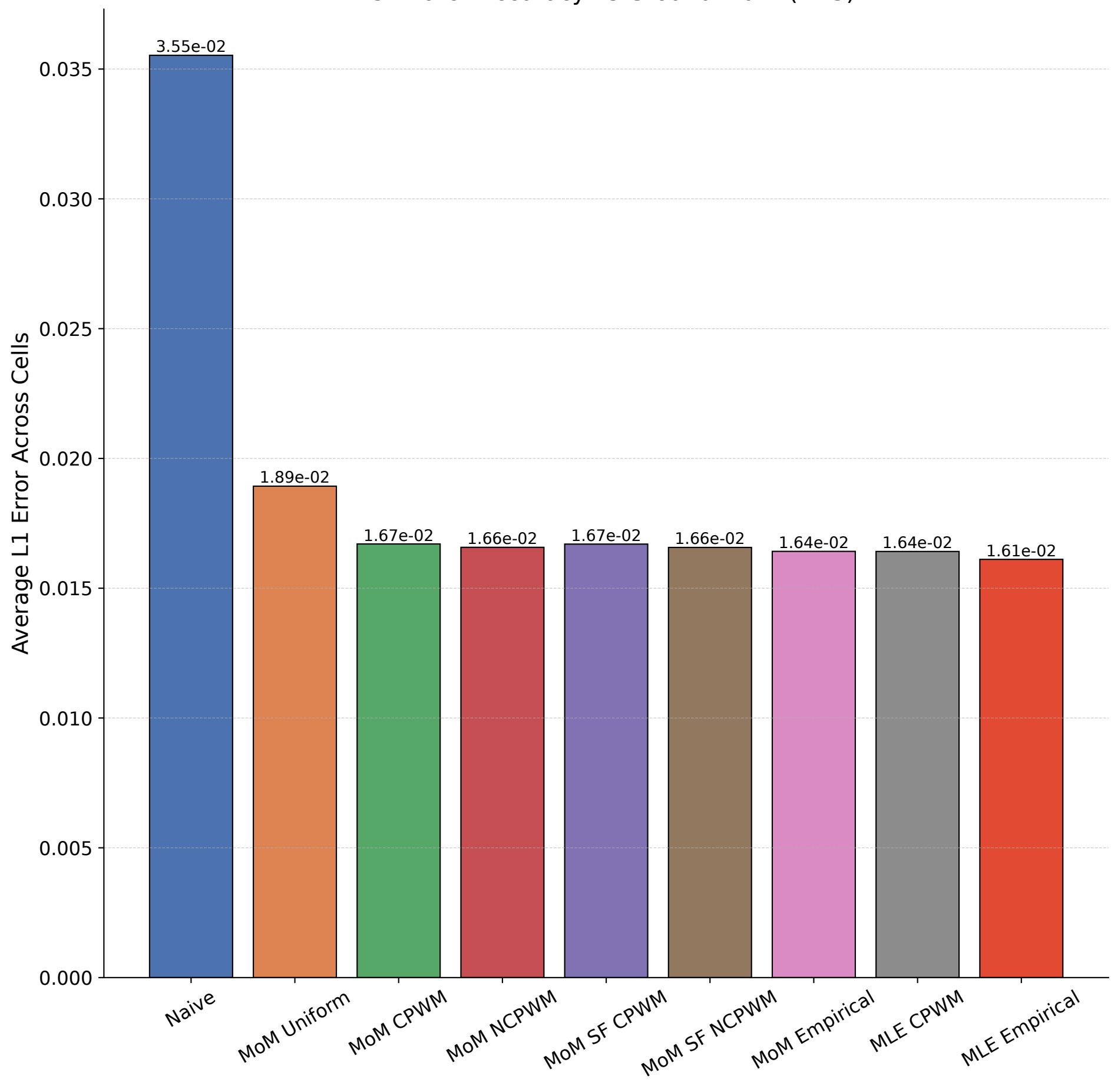
Estimator Accuracy vs Ground Truth (k=5)
