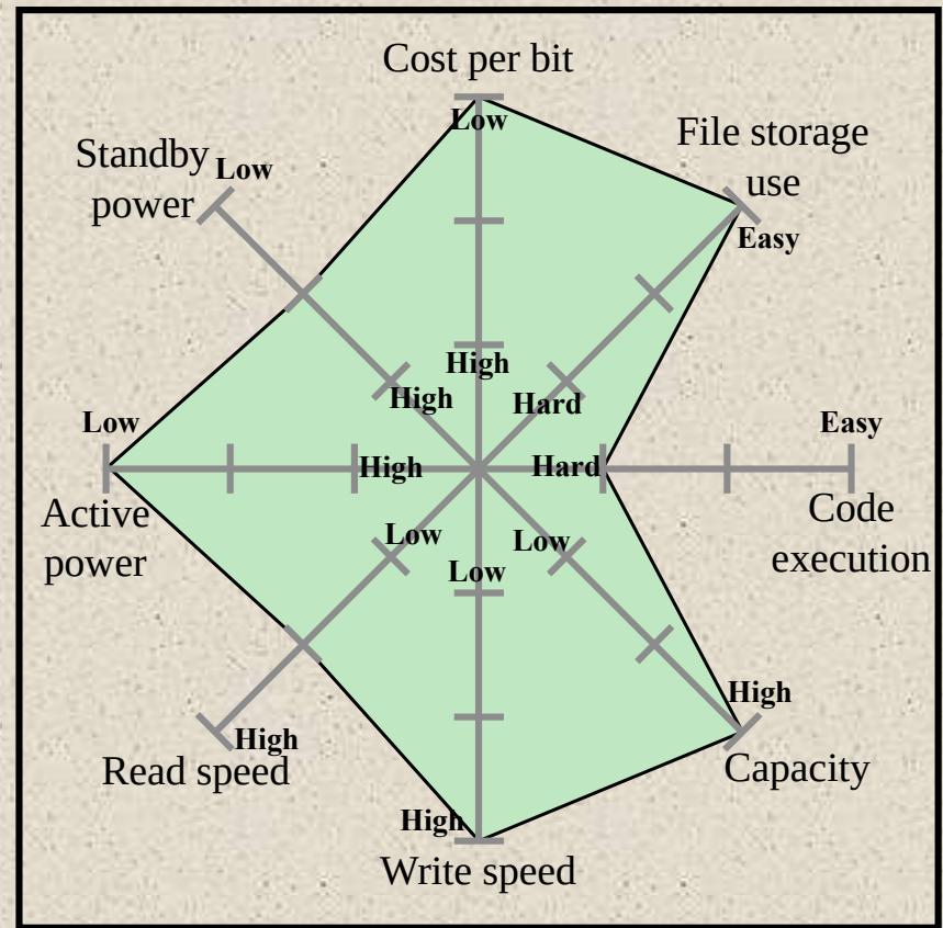
(b) NAND
