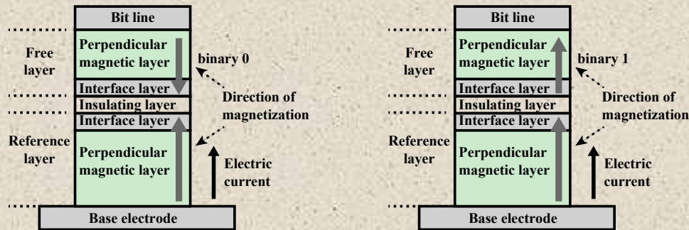
(a) STT-RAM
