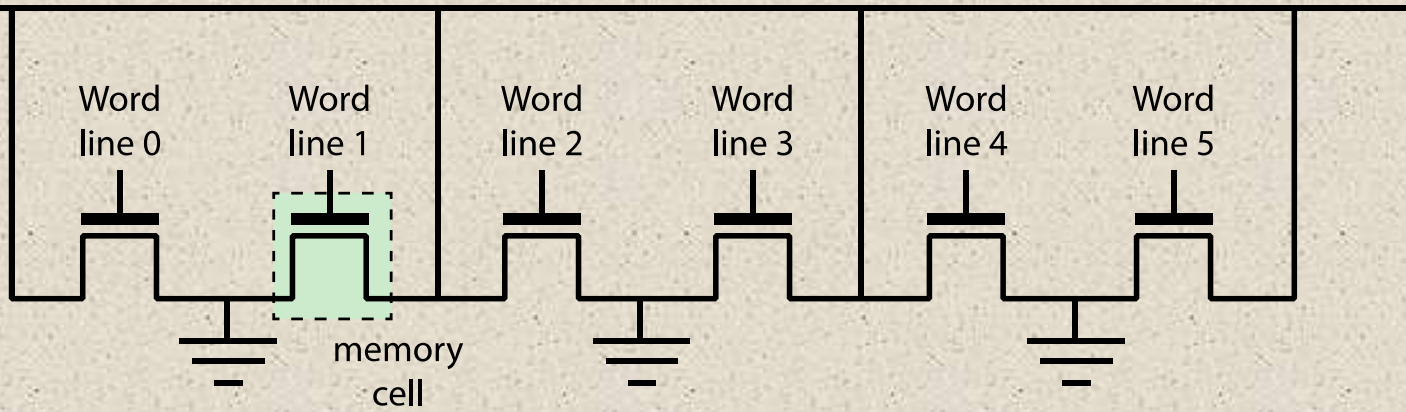
(a) NOR flash structure
