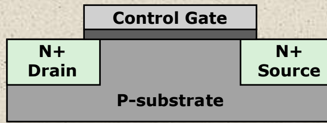
(a) Transistor structure
