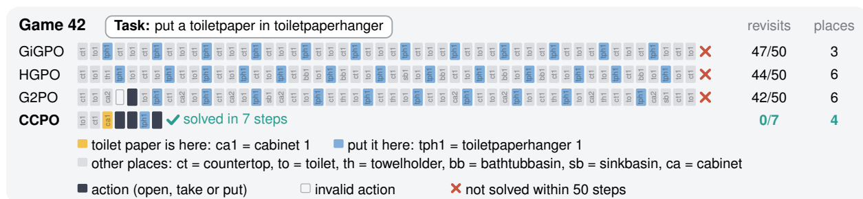
Figure S2 Evaluation trajectories for the navigation task in Table S6. Reproduced from Figure 3. Each cell denotes one step; revisit counts track navigation to previously visited locations. CCPO uses A_{CC} only.
