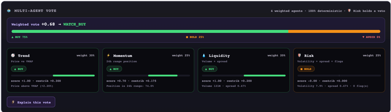
Figure 3 — Multi-Agent Vote: weighted bars, per-agent cards, and the Risk veto.
