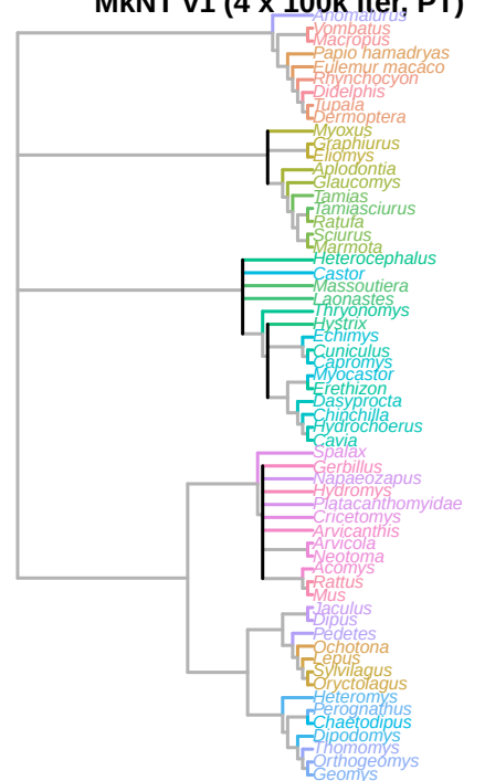
BLIND MR consensus (N=1893) MkNT v1 (4 x 100k iter, PT)
