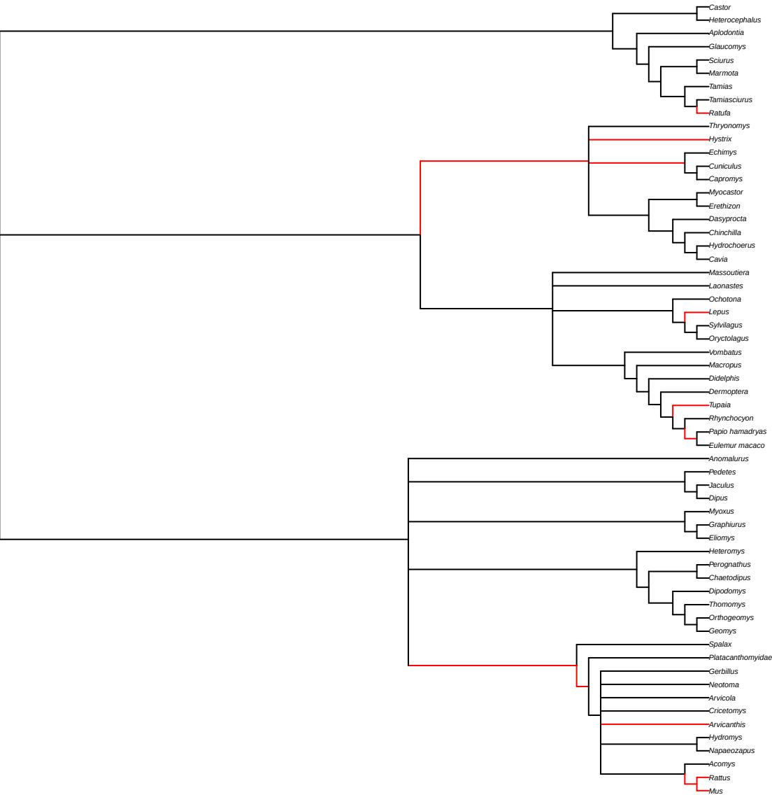
AWARE MR consensus (N=120 post-burnin) (red = aware-unique splits)
