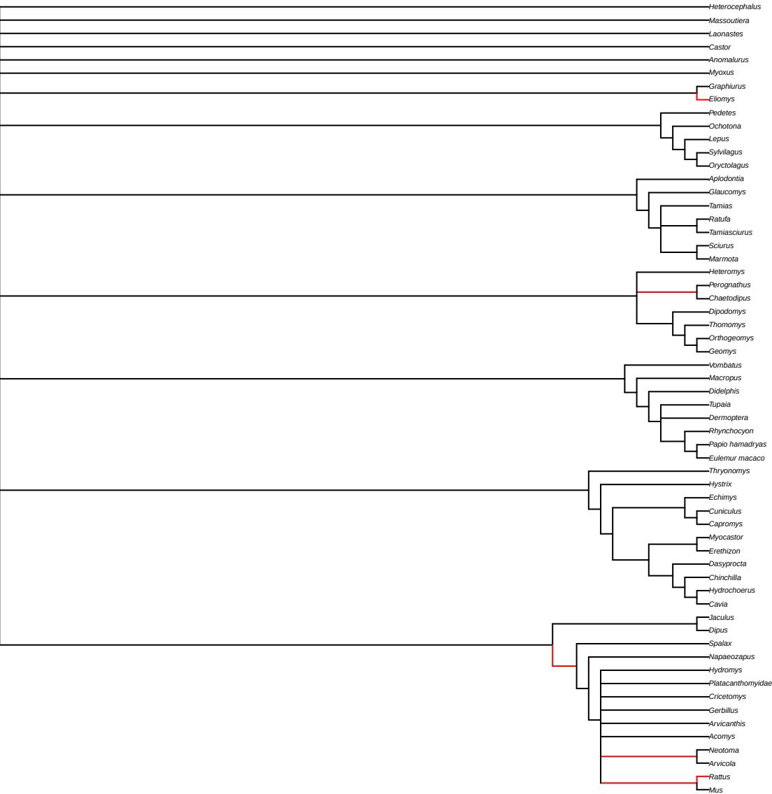
BLIND MR consensus (N=269 post-burnin) (red = blind-unique splits)
