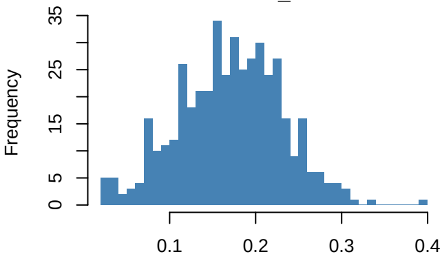
phi theta_1
