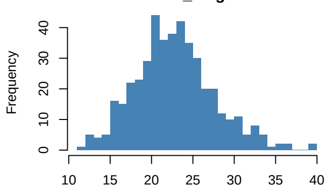
pi0 tree_length
