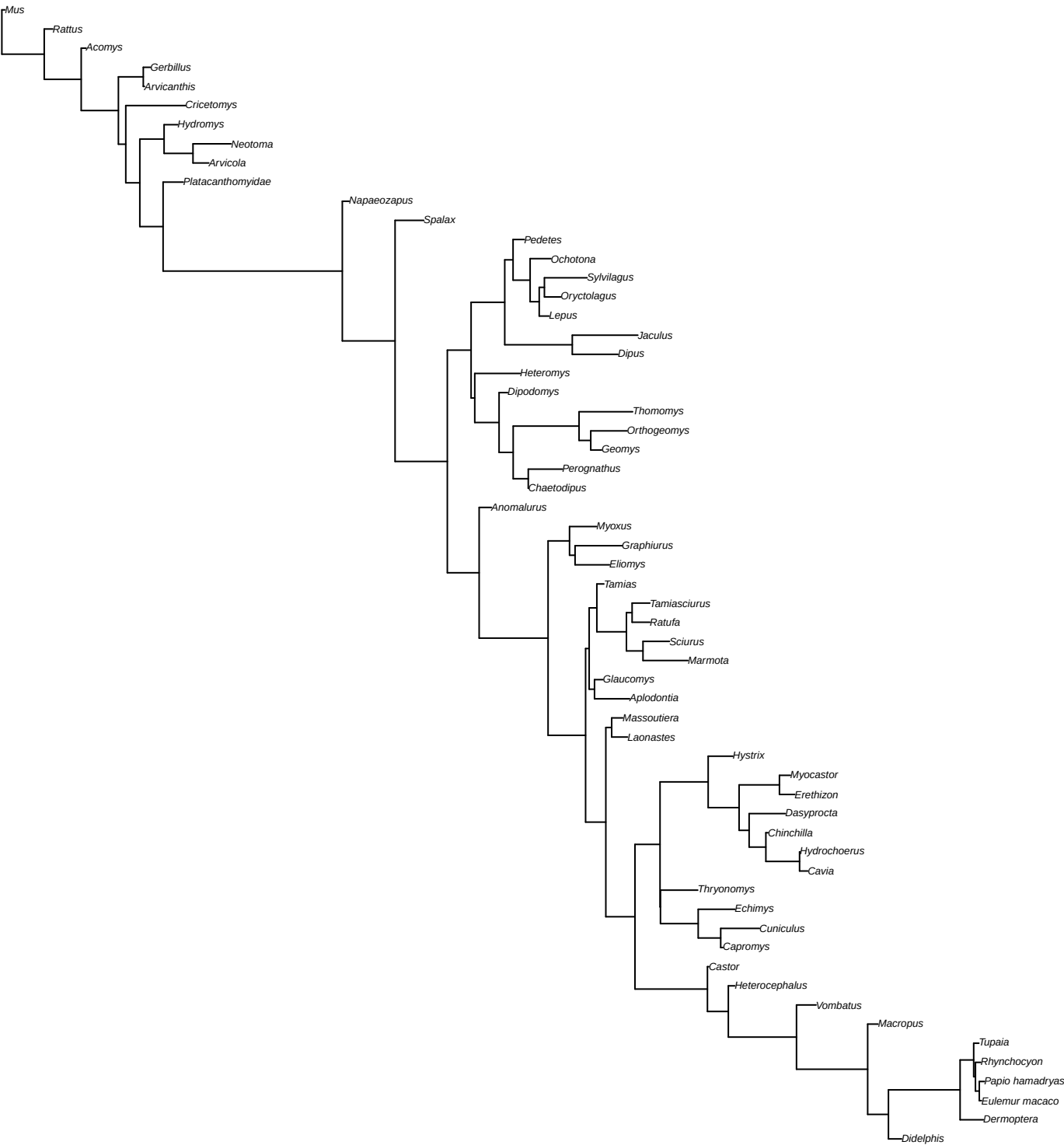
BLIND one-sample phylogram (TL=18.5, mean edge=0.157)
