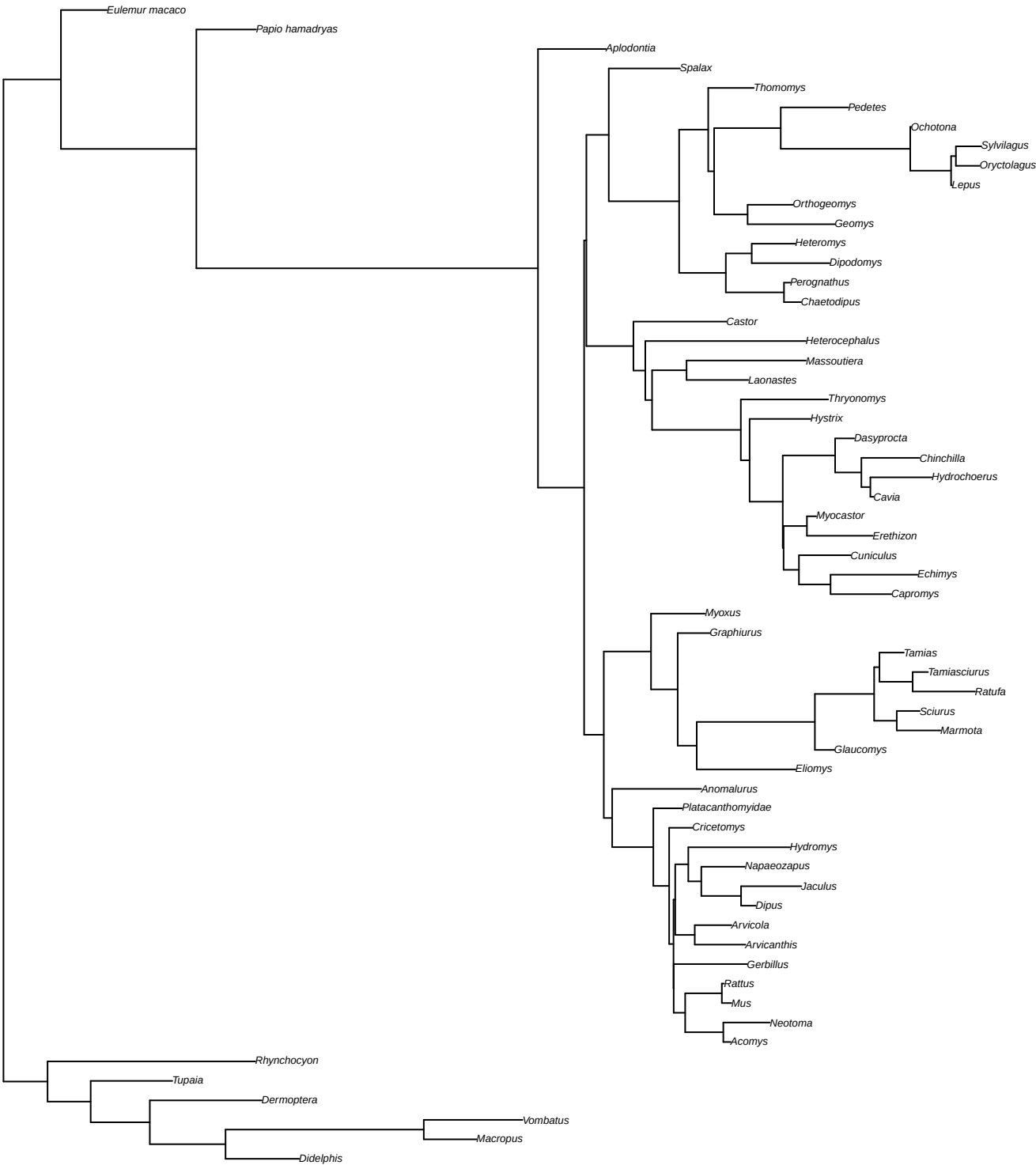
AWARE one-sample phylogram (TL=18.6, mean edge=0.158)
