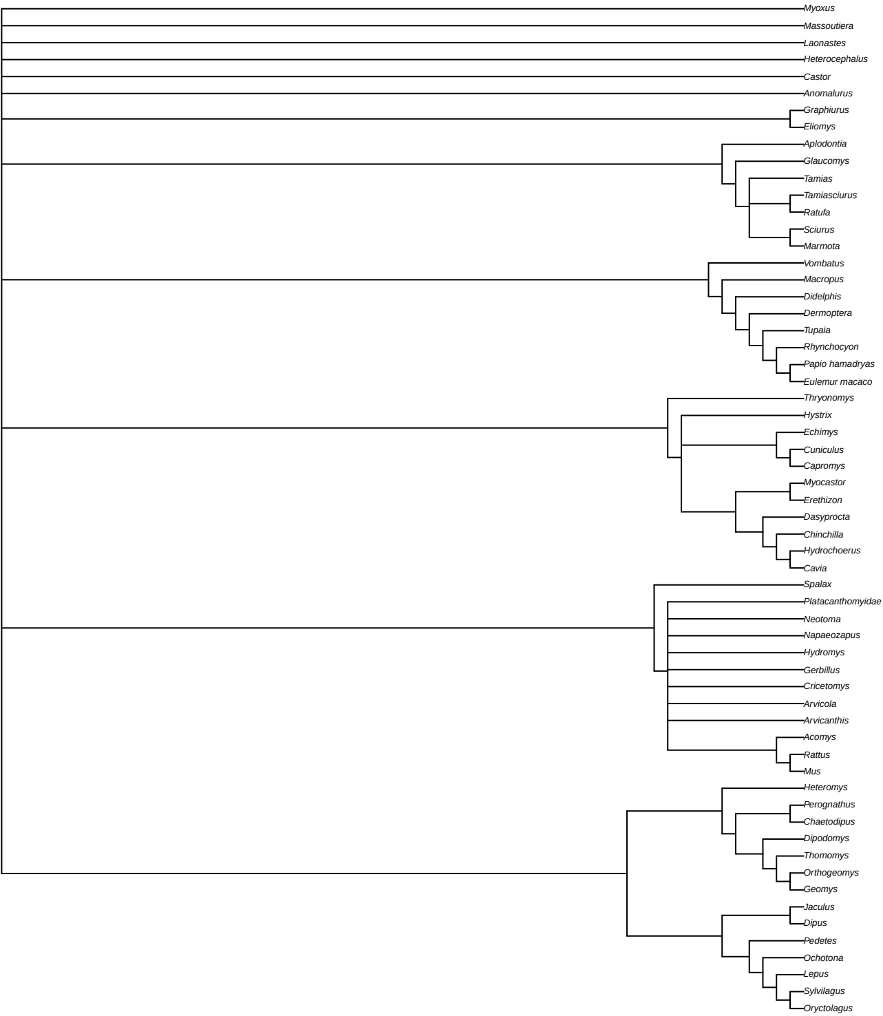
BLIND consensus (n=3869, TL=18.5)
