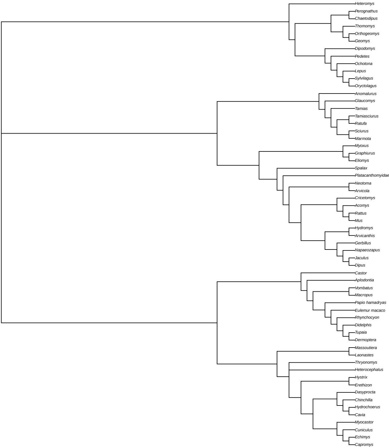
AWARE consensus (n=93, TL=18.7)
