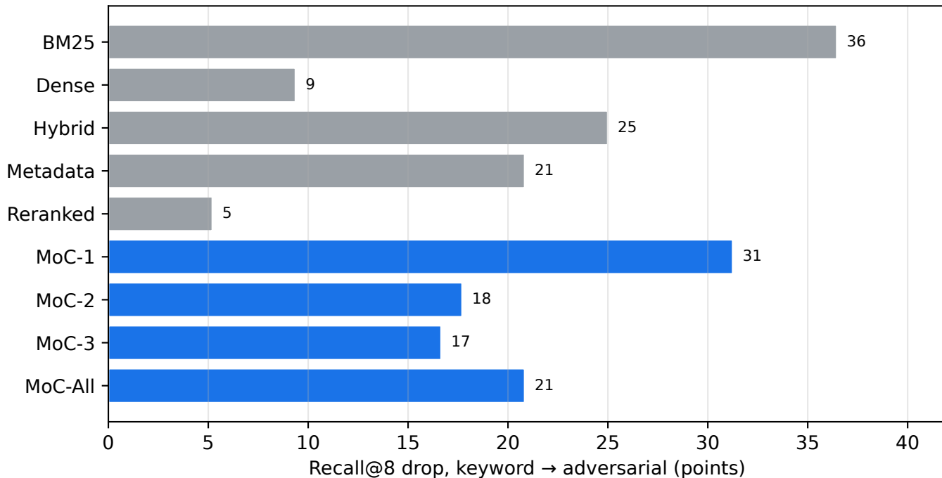
Recall drop under adversarial shift (lower is better)
